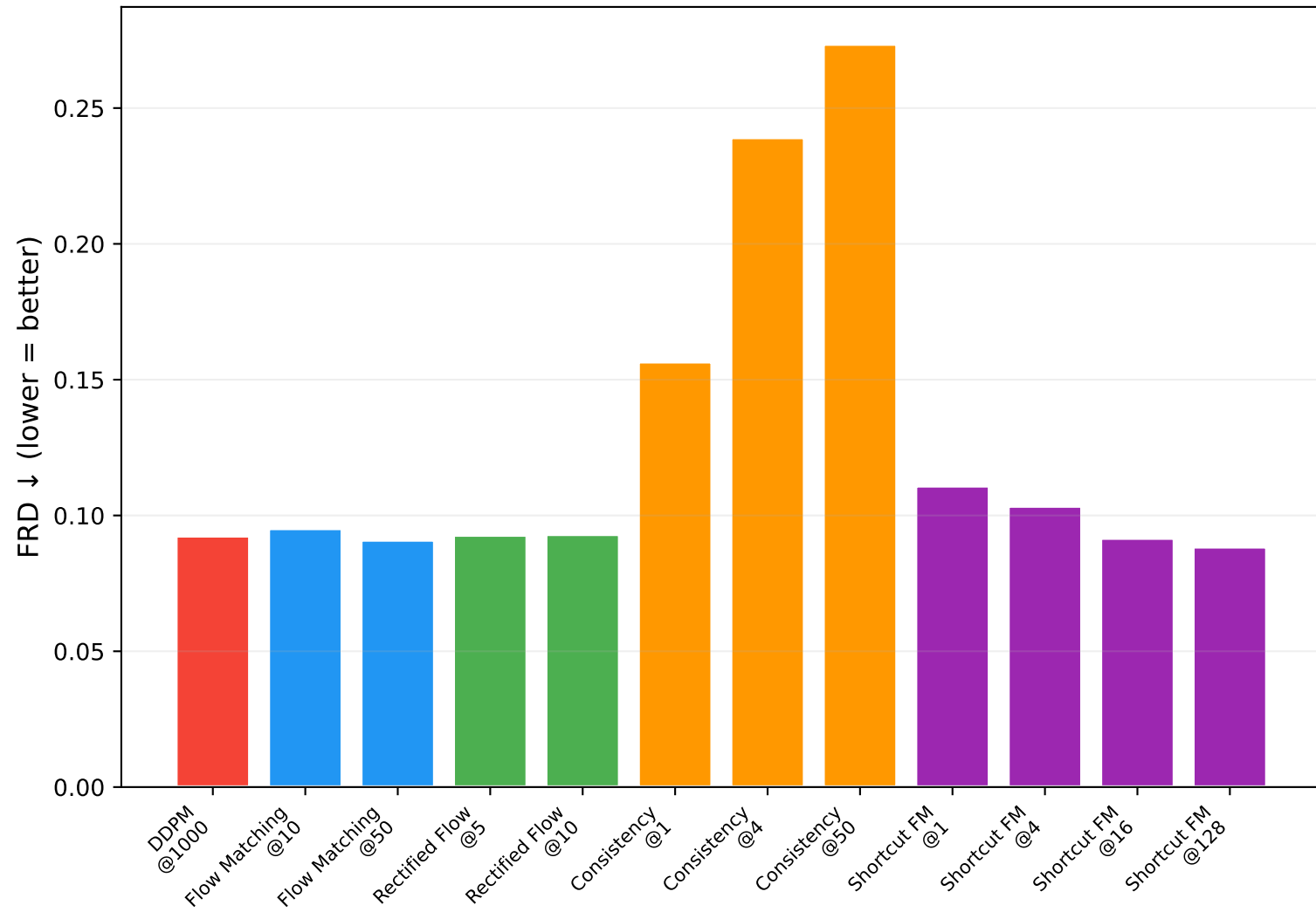
(a) Fréchet Radiomic Distance
