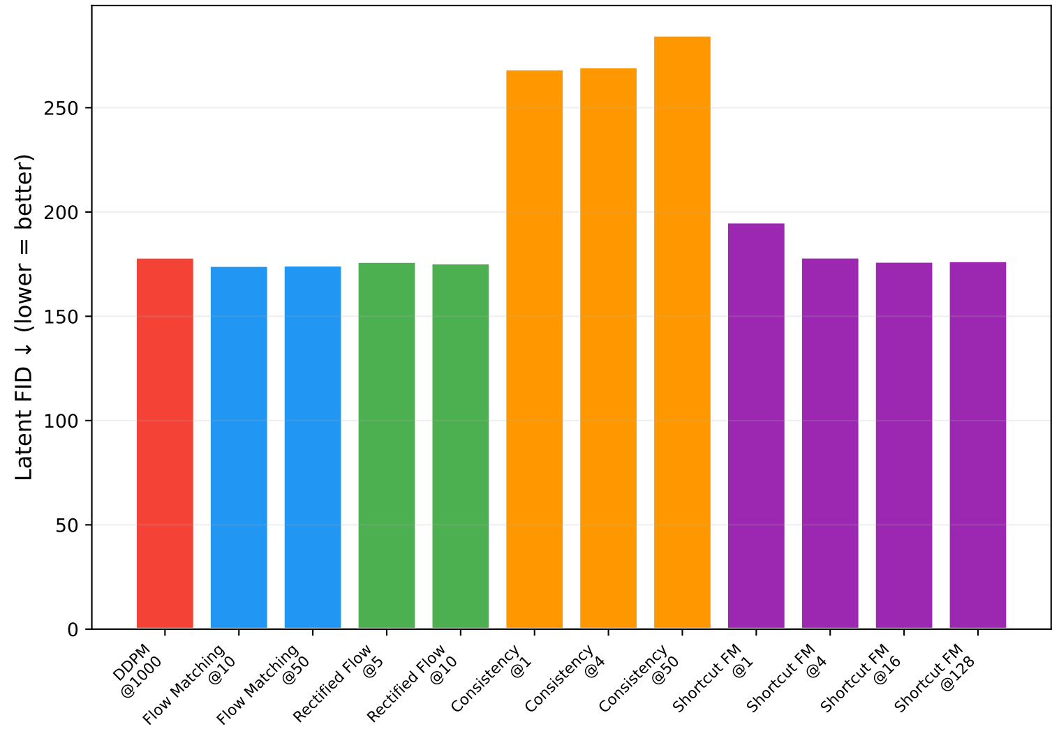
(b) Fréchet Distance in VQ-GAN Latent Space
