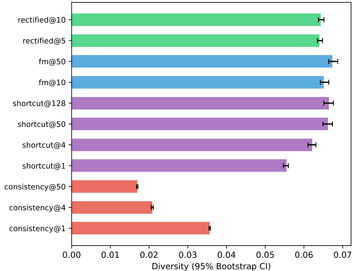
Diversity (L1 pairwise)
