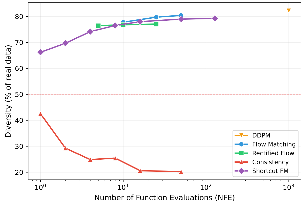
Diversity vs Inference Steps
