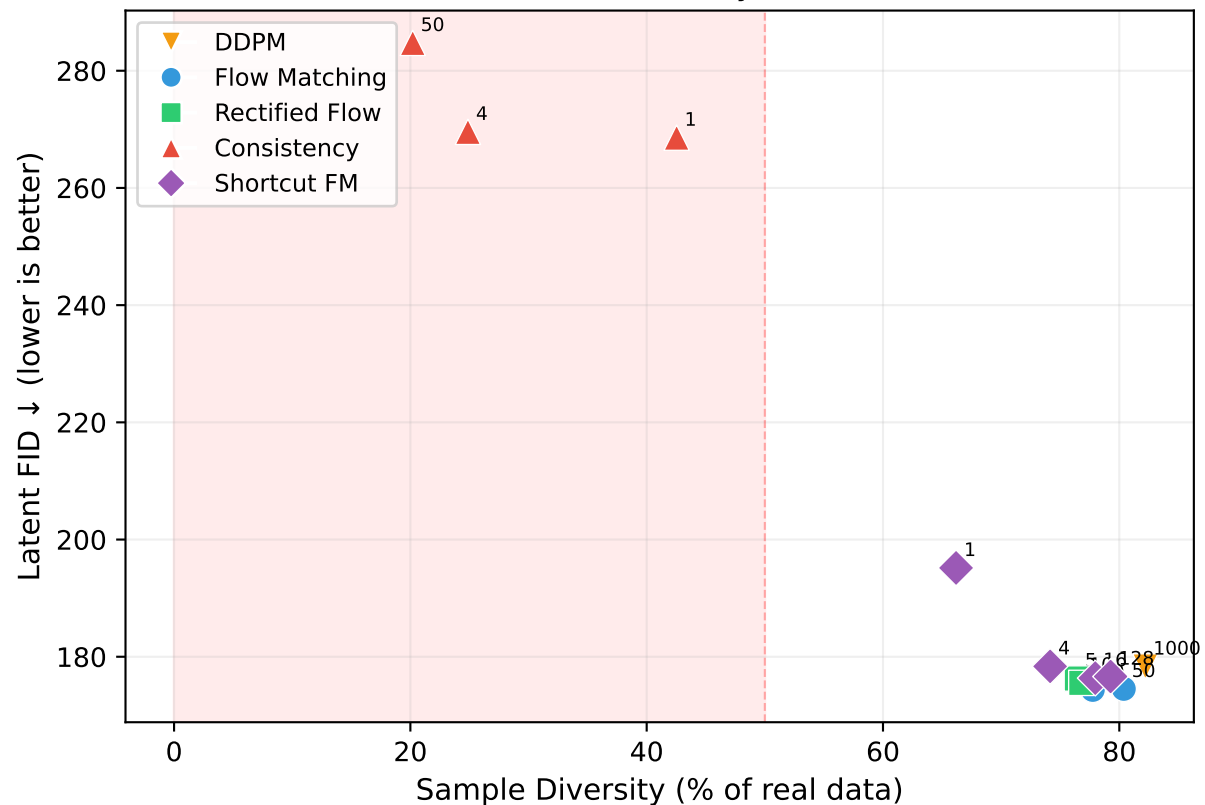
Latent FID-Diversity Frontier
