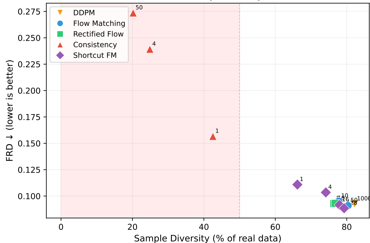
Distributional Quality-Diversity Frontier
