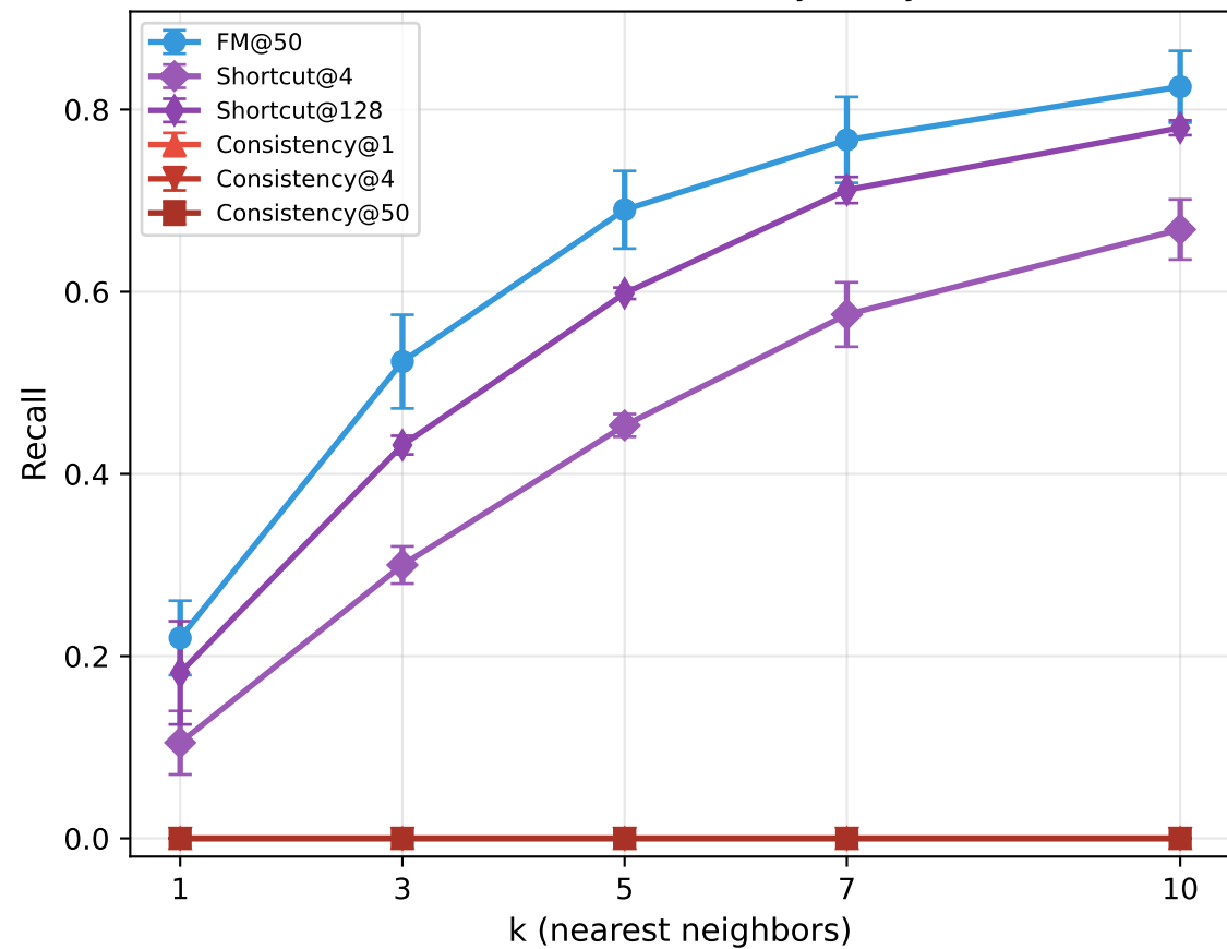
Recall vs k — Sensitivity Analysis
