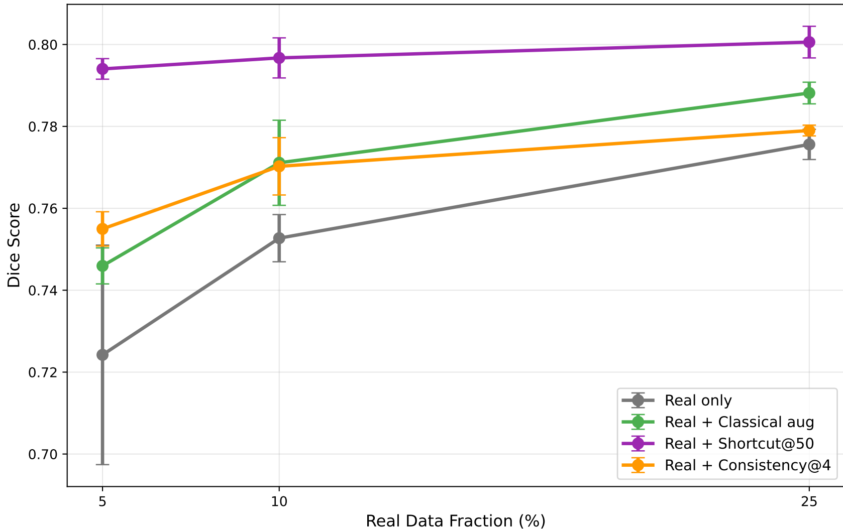
Downstream Tumor Segmentation: Augmentation Strategy Comparison
