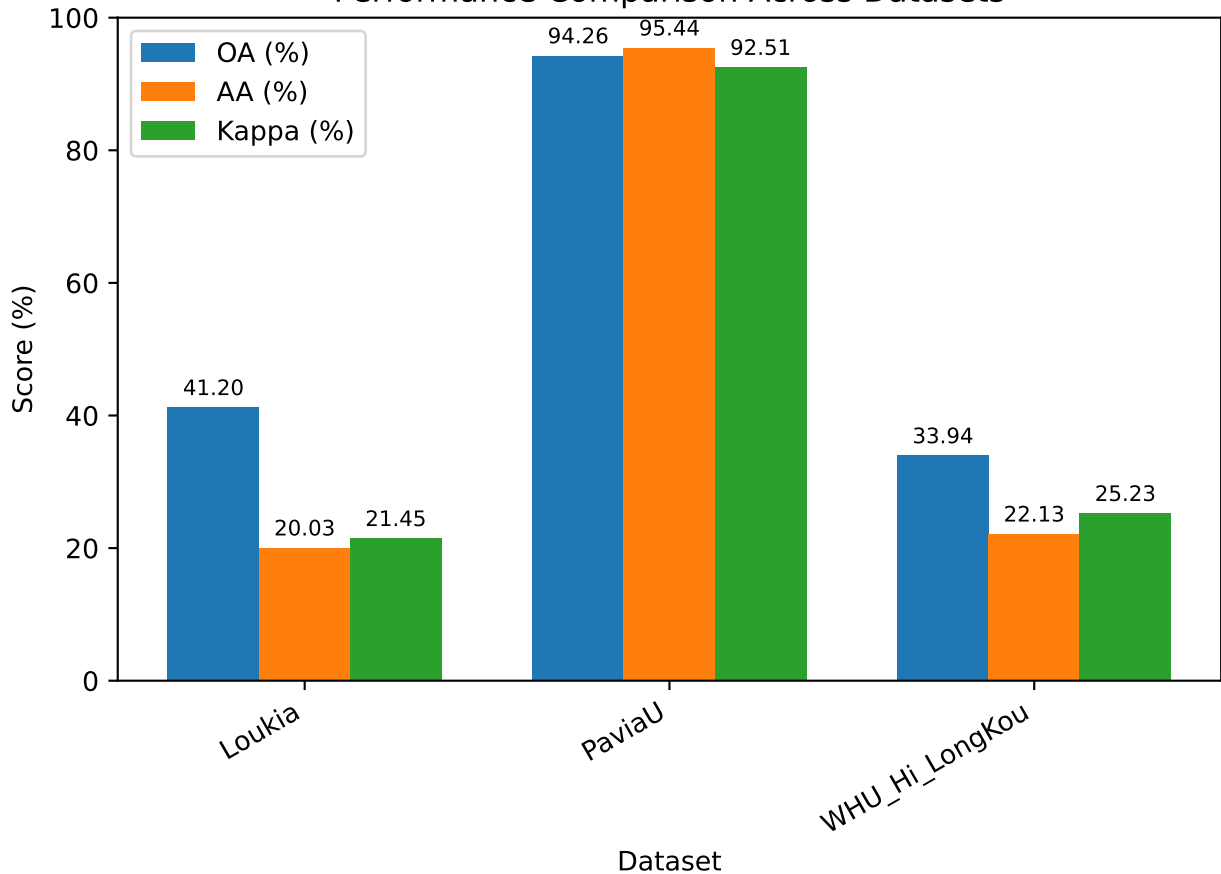
Performance Comparison Across Datasets
