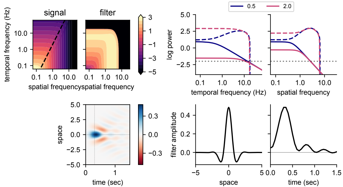
Figure 3: Optimal filter and kernel.
