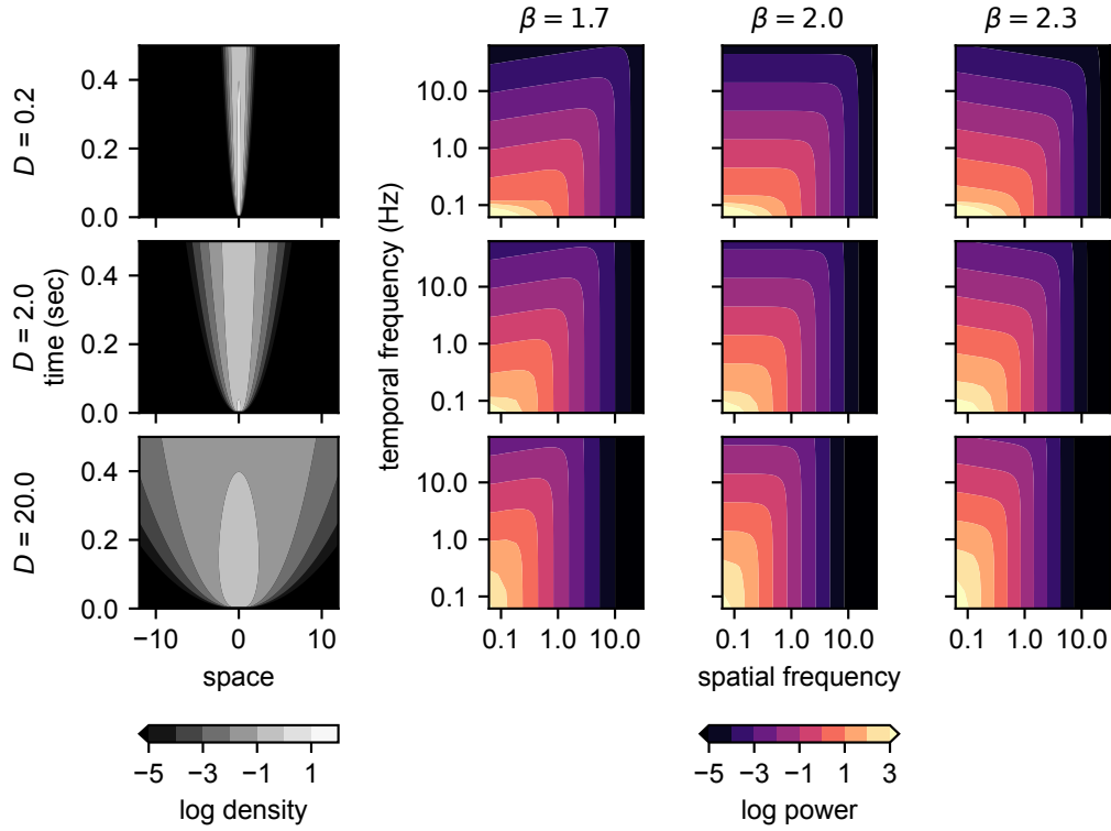
Figure 1: Spatial and temporal spectra for different betas.
