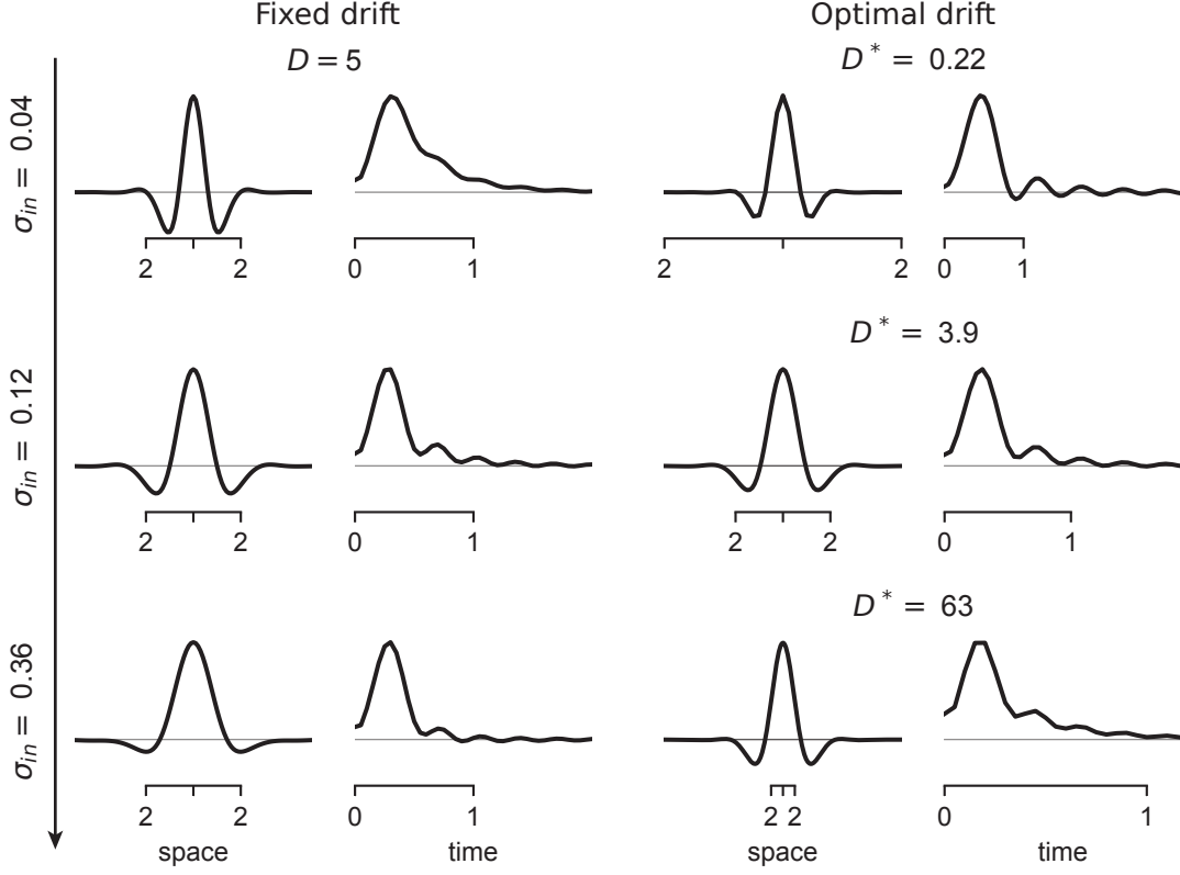
Figure 4: Optimal filter and kernel.
