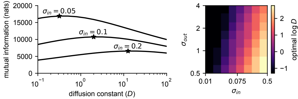
Figure 2: Optimal diffusion constant vs. input and output noise.
