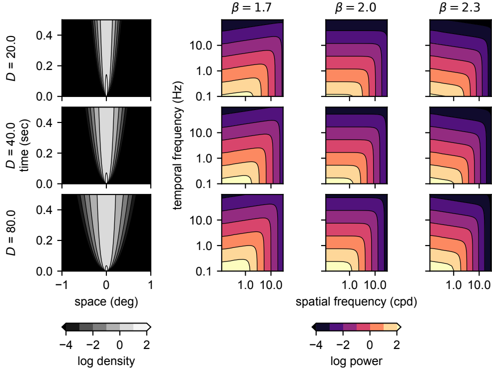
Figure 2: spatio temporal power spectra for different betas. Diffusion values are in \text{arcmin}^2/\text{s} .
