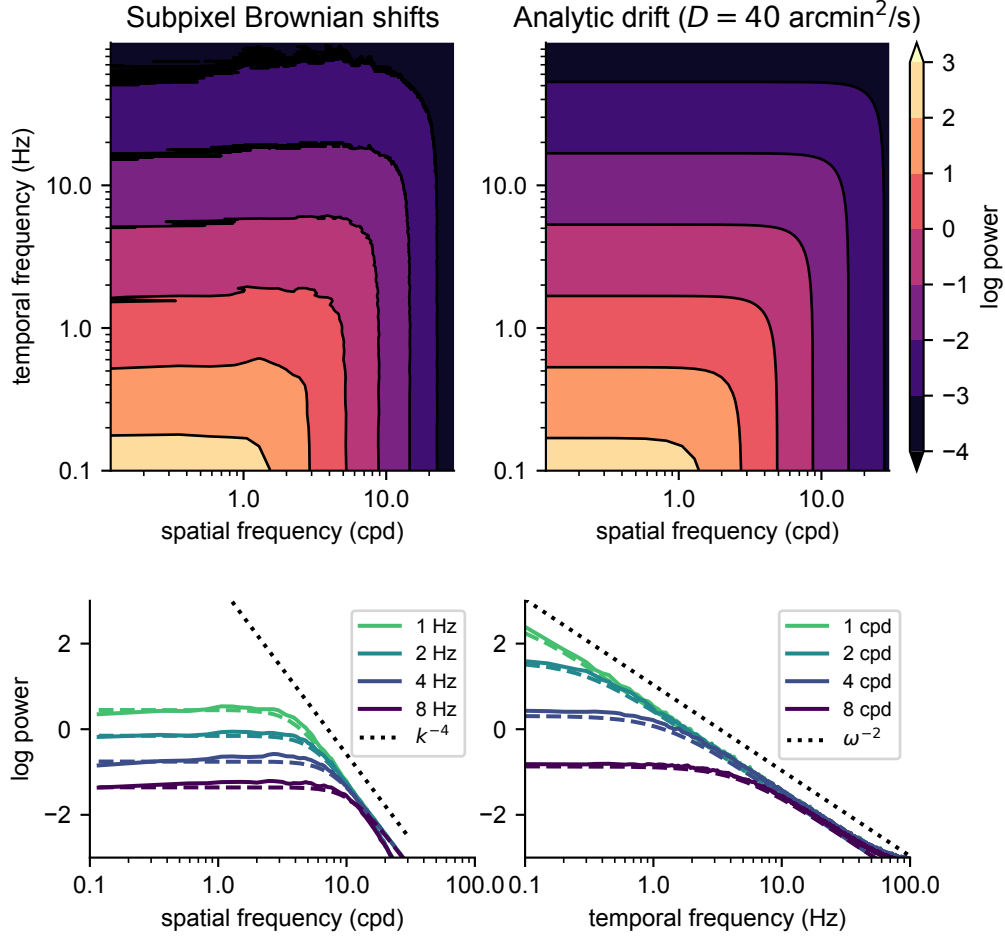
Figure 1: Drifting natural images and analytic model are in good agreement.
