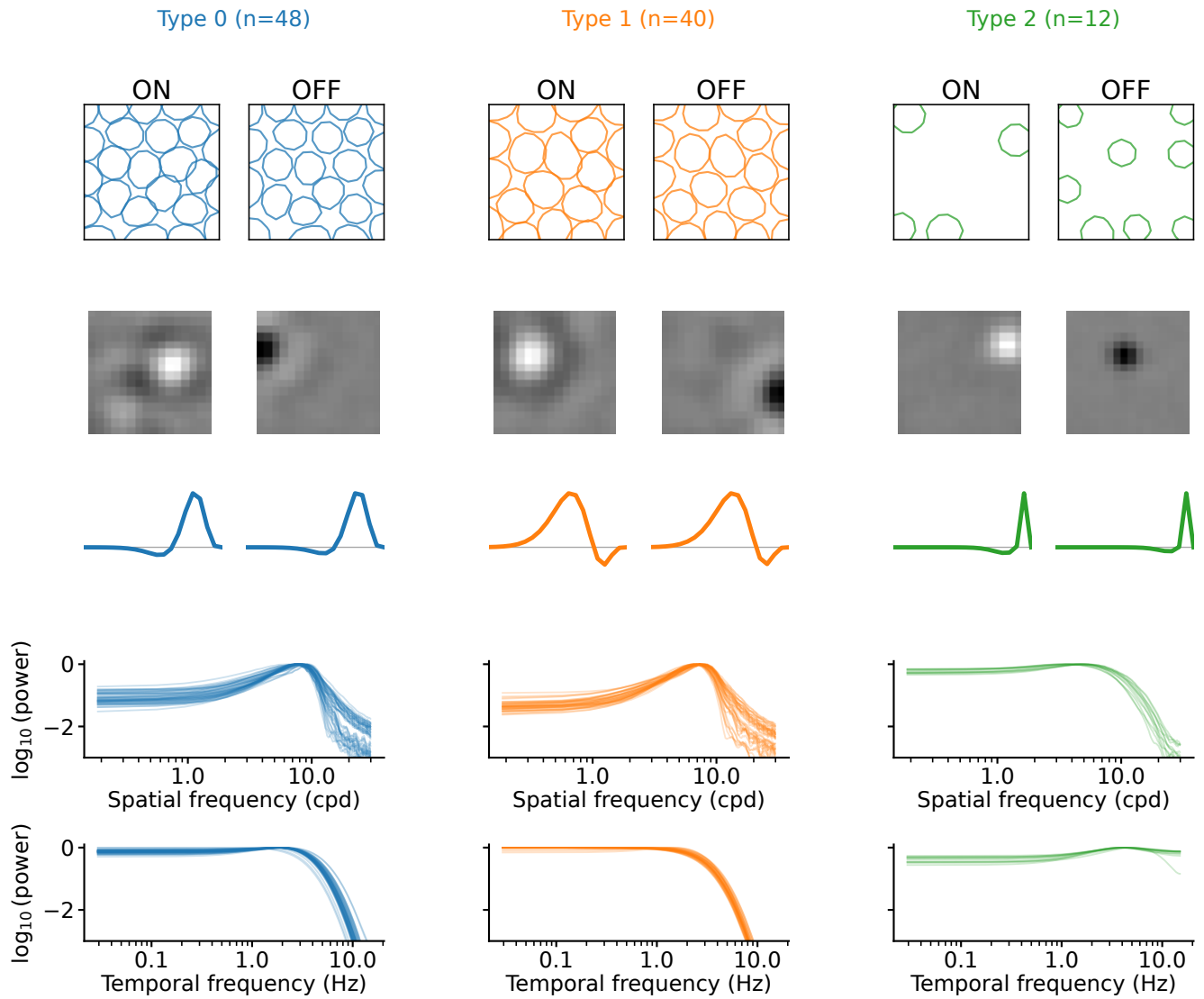
Figure 5: Optimal weights for linear nonlinear model.
