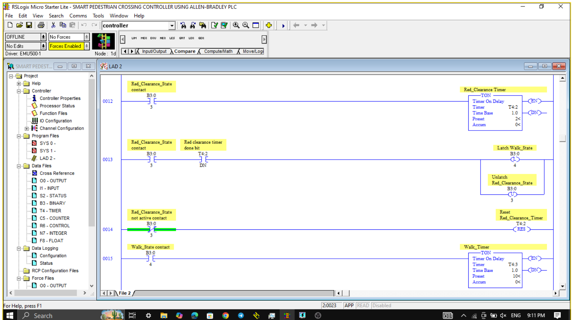
Figure 6: Red clearance state timer and transition to walk state.
