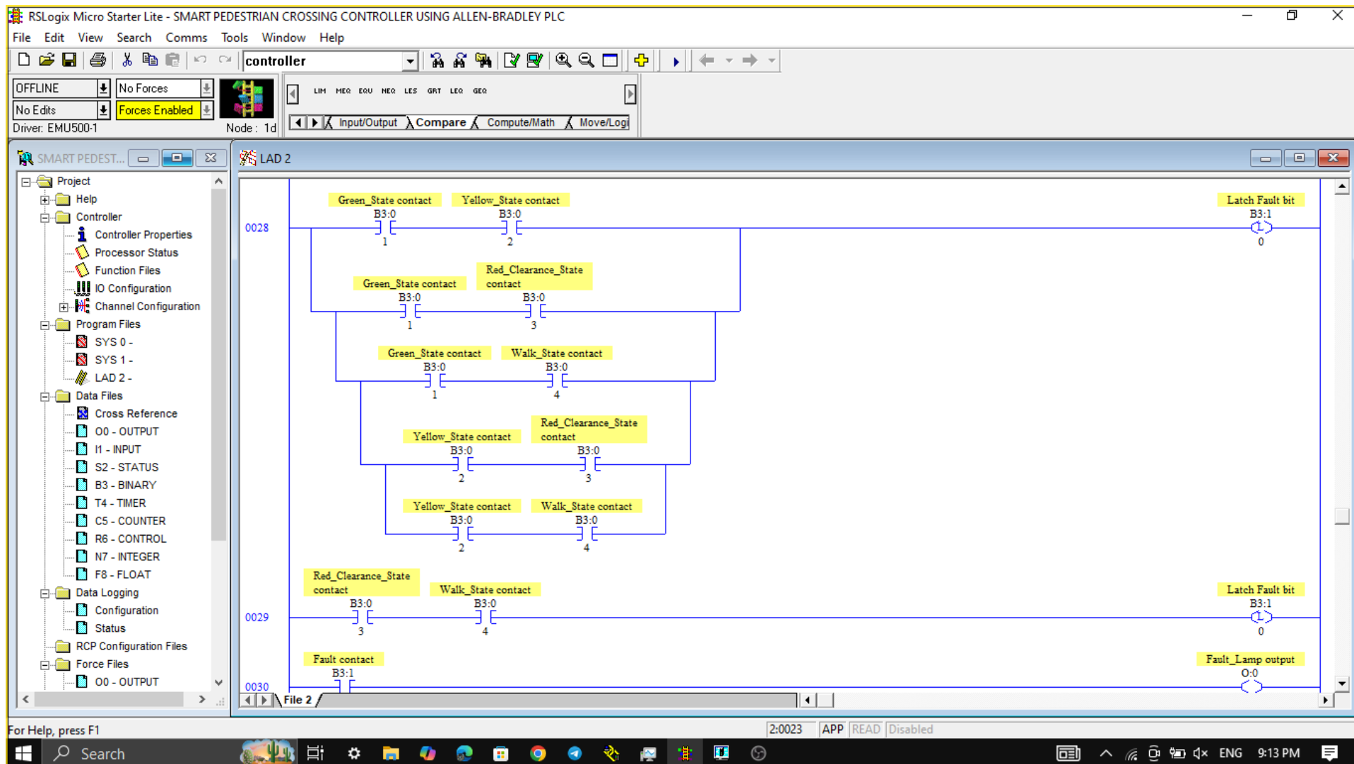
Figure 11: Fault detection logic and fault lamp output.
