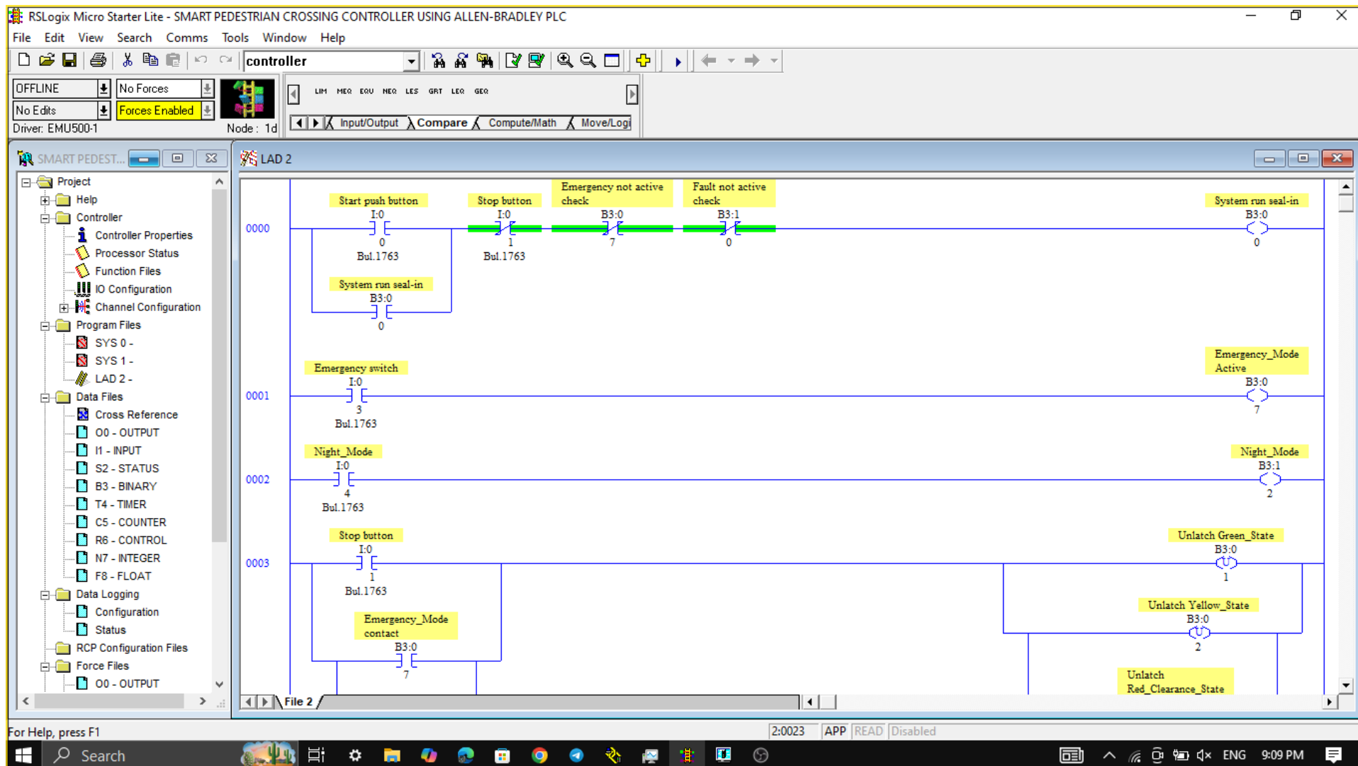
Figure 1: Start, stop, emergency, and night mode input logic.
