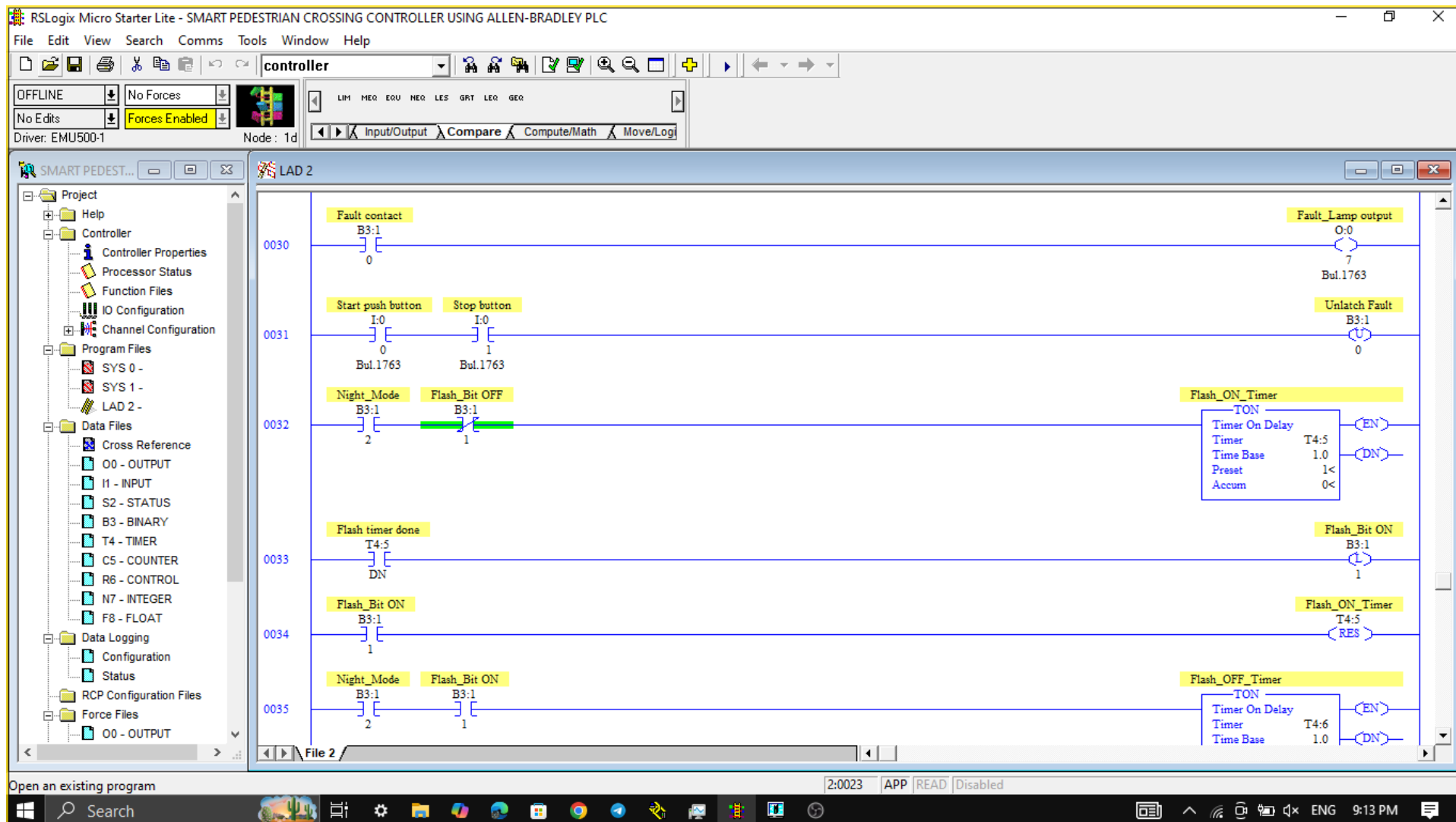
Figure 12: Flash ON timer and flash bit generation logic.
