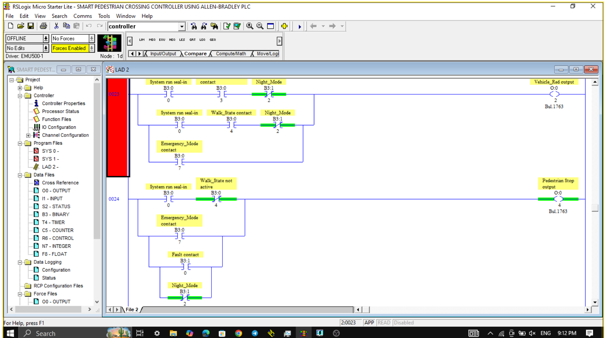
Figure 9: Vehicle red output and pedestrian stop output logic.
