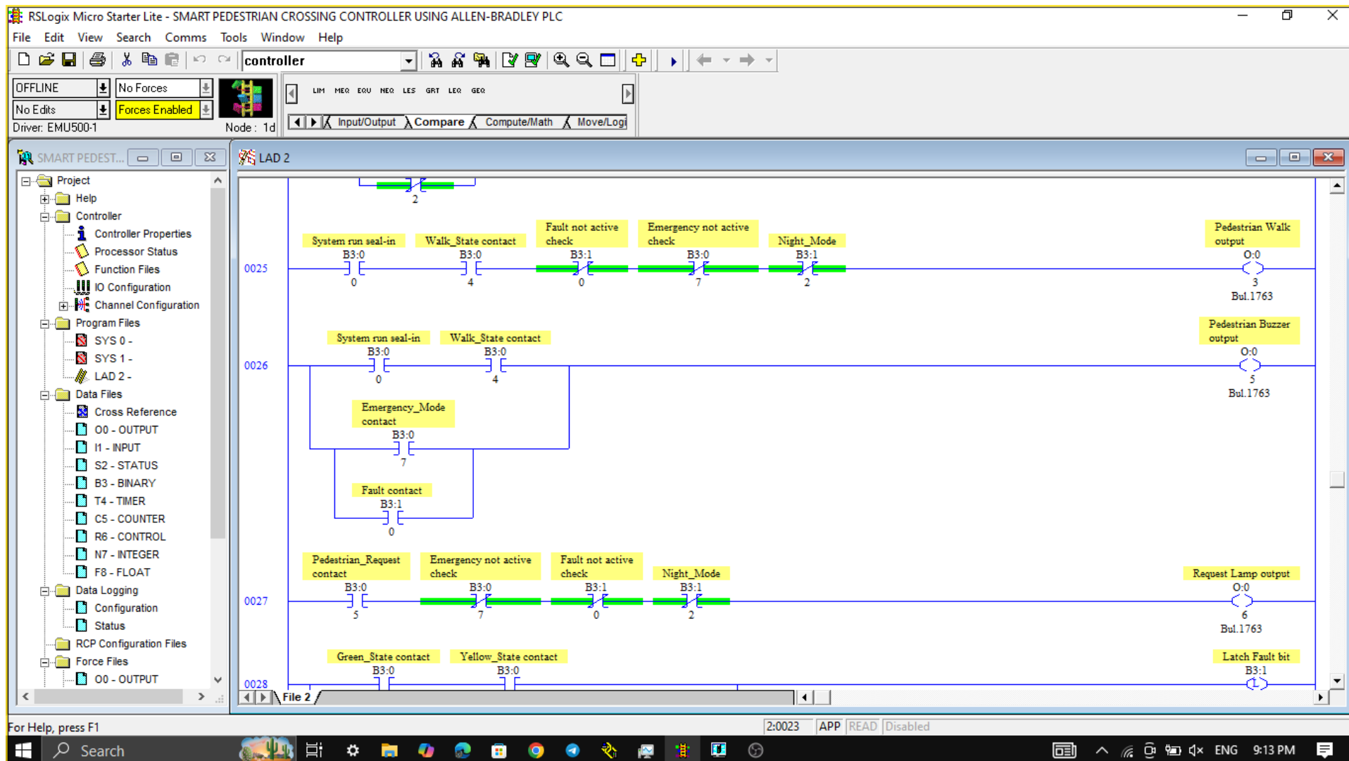
Figure 10: Pedestrian walk, buzzer, and request lamp output logic.
