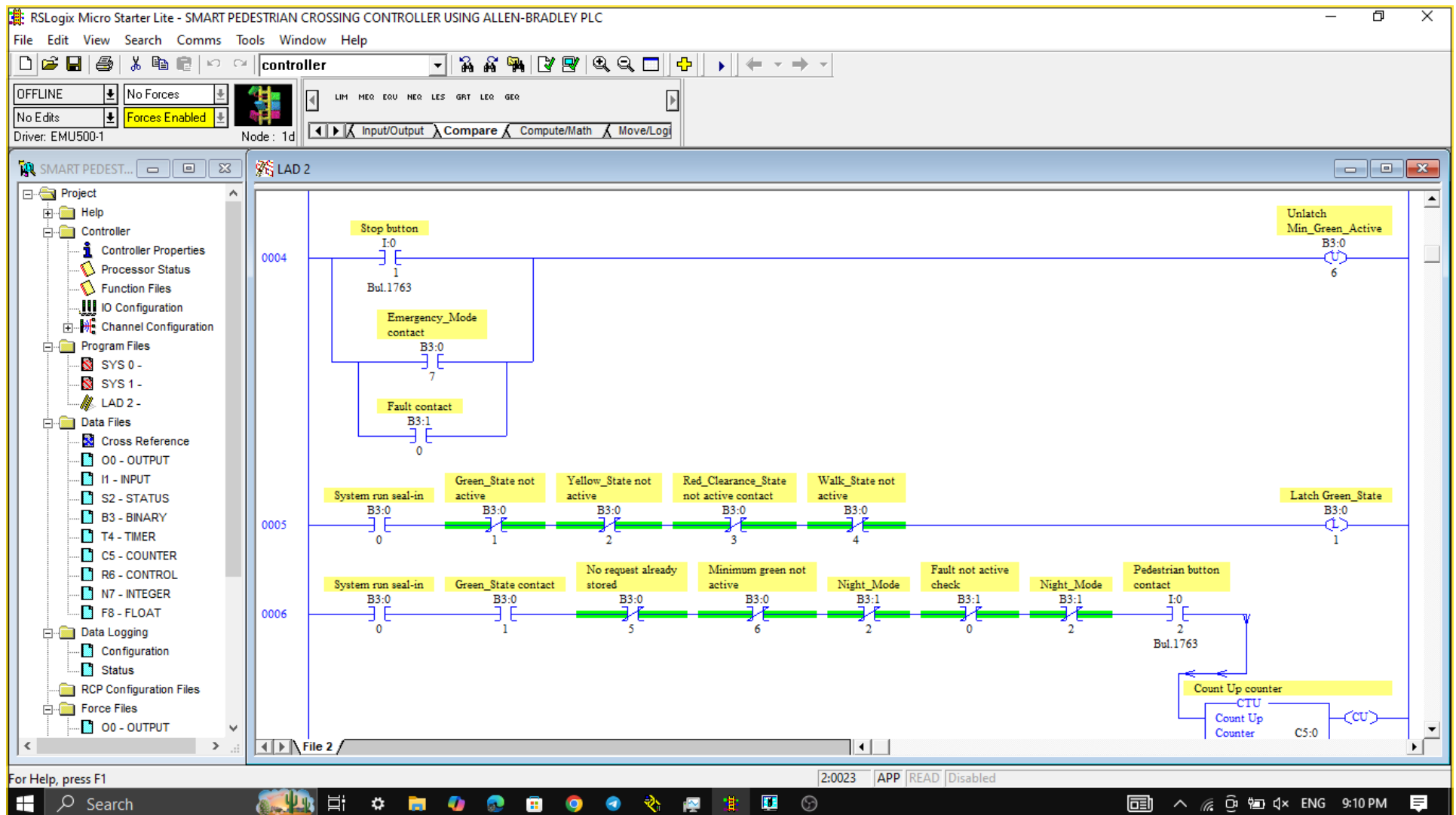
Figure 3: Green state latch and pedestrian request counter logic.
