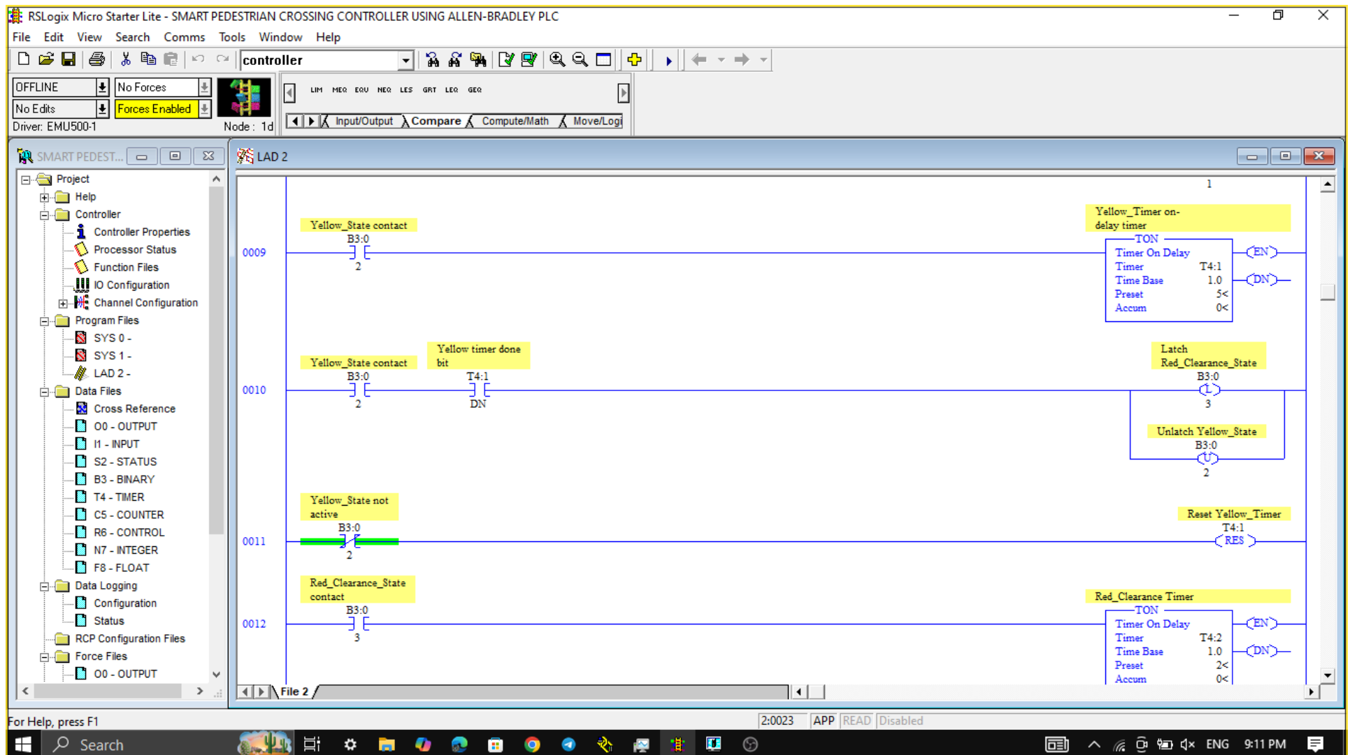
Figure 5: Yellow timer, yellow-to-red transition, and red clearance timer.
