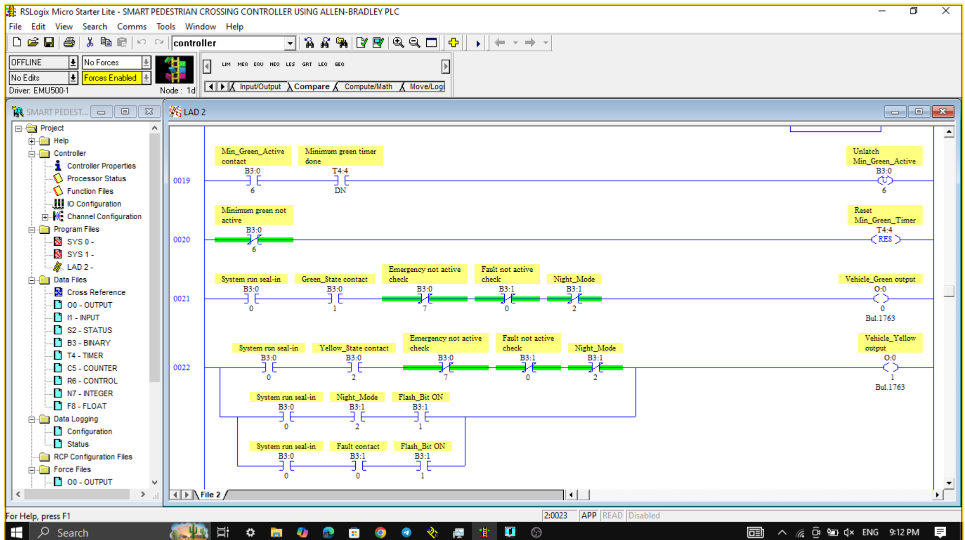
Figure 8: Vehicle output logic including green, yellow, night flash, and fault-related yellow blinking.
