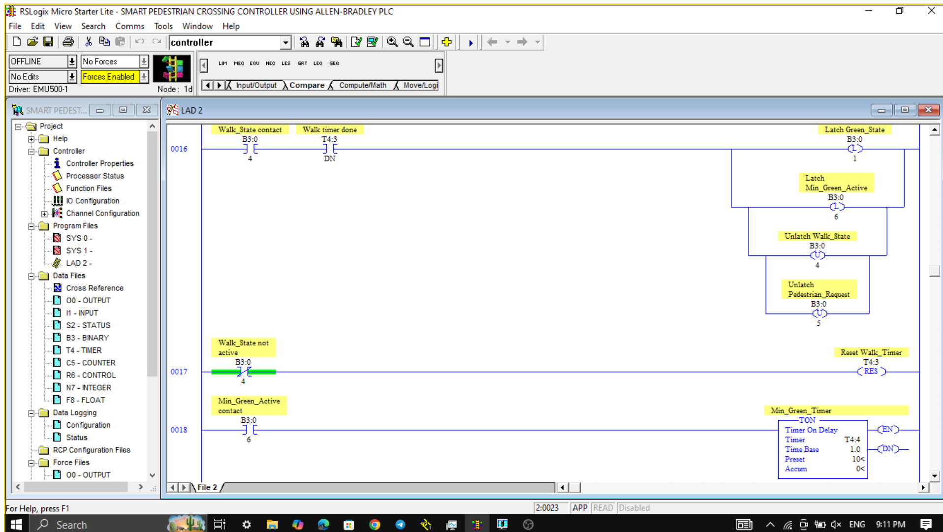
Figure 7: Walk timer completion, return to green state, and reset logic.
