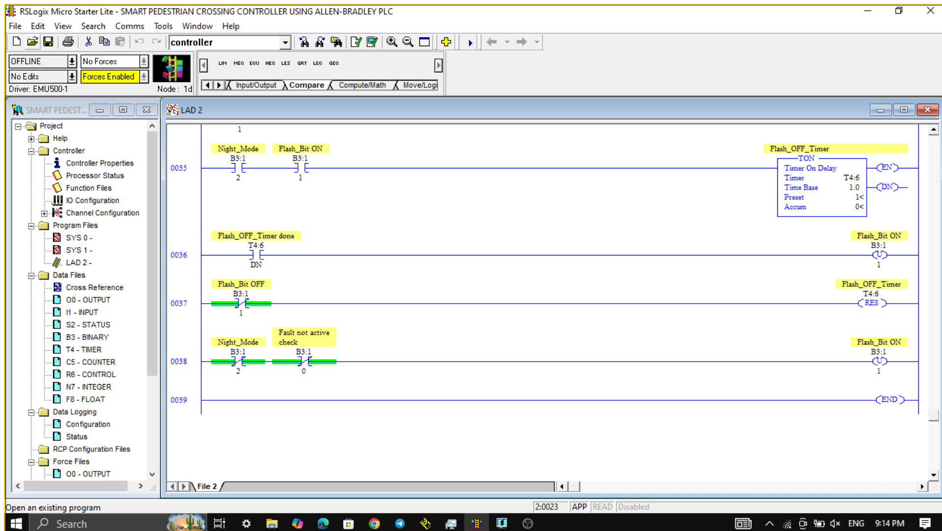
Figure 13: Flash OFF timer and end of ladder program.
