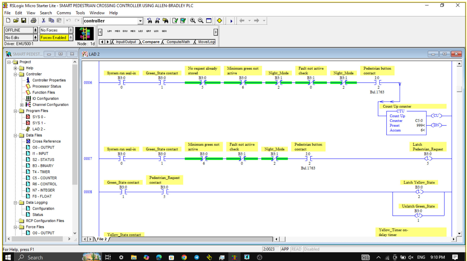
Figure 4: Pedestrian request latch and transition from green state to yellow state.
