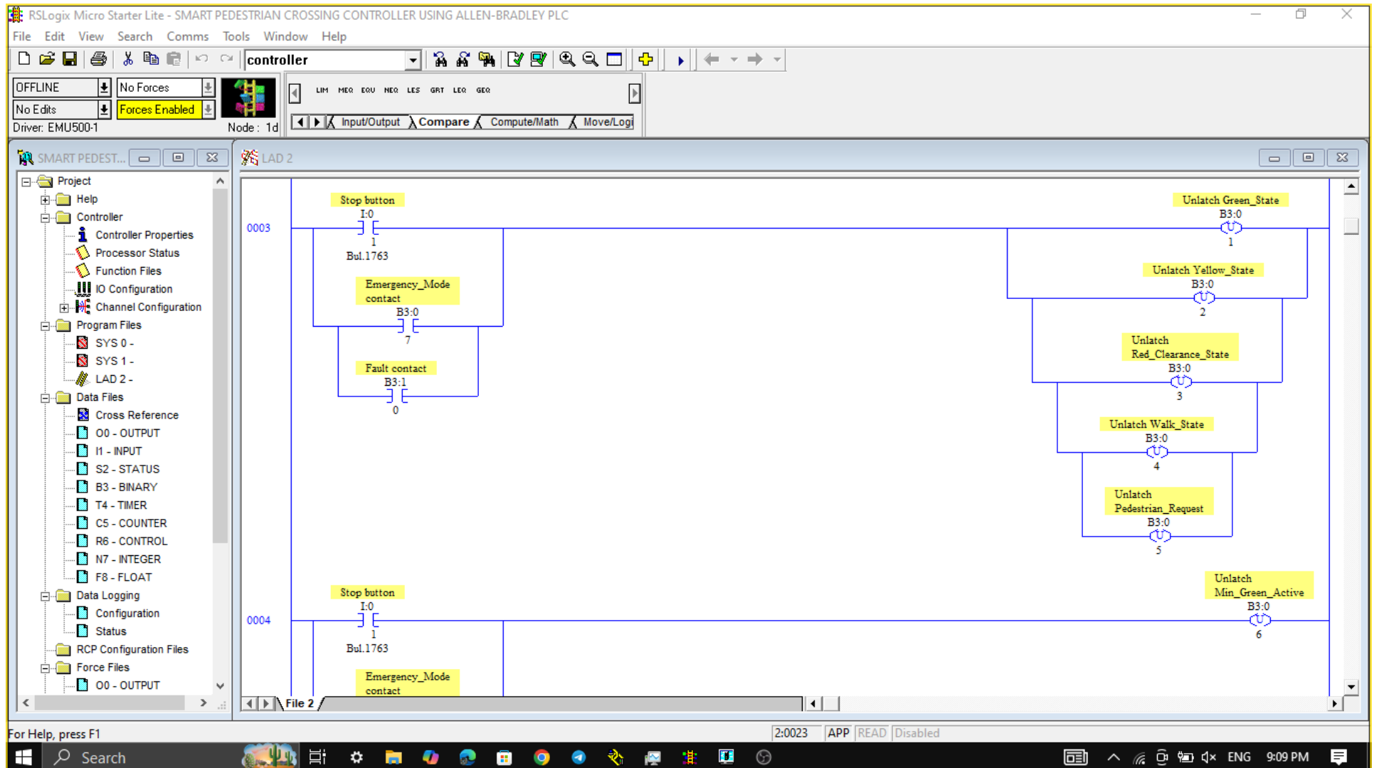
Figure 2: Stop, emergency, and fault reset logic for internal states.
