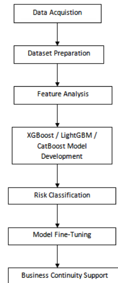
Fig. 1. Workflow of Predictive Analytics for Business Resilience Systems Integrating AI Systems (BRS + AIS)
