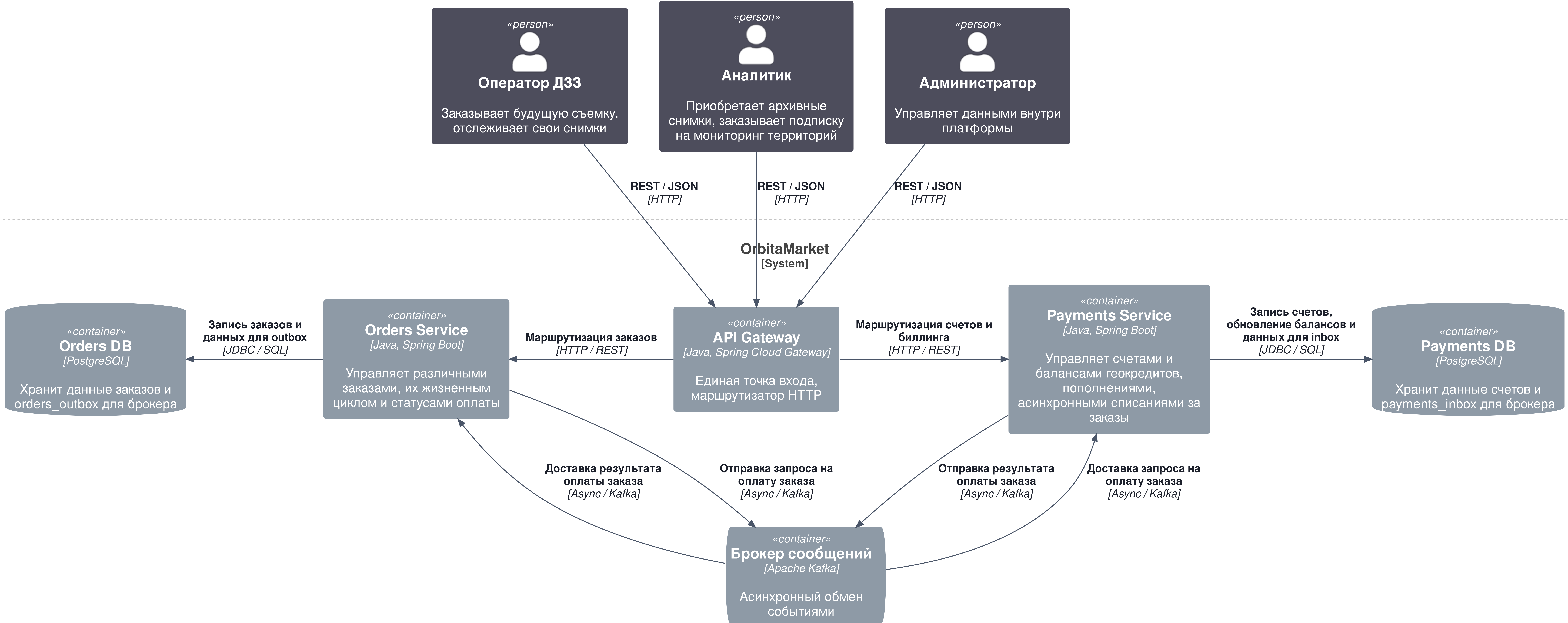
[OrbitaMarket] C2 — Container Diagram
