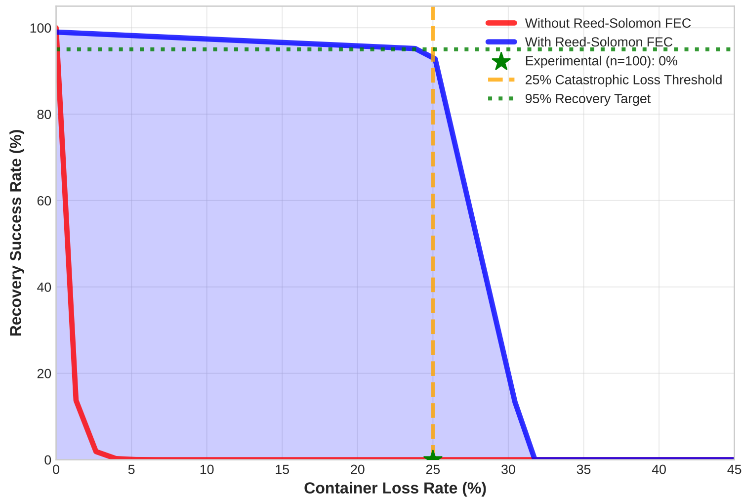
A) Reed-Solomon Error Correction Performance vs Container Loss Rate
