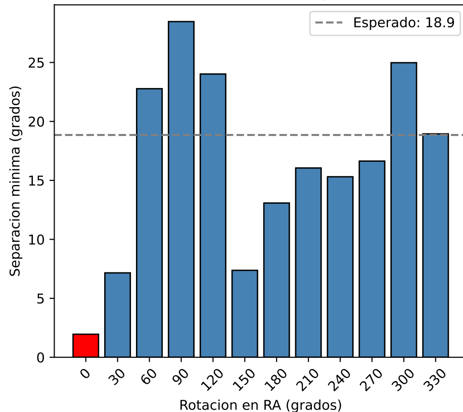
GW190814-SGP: 2.0 deg (unico)
