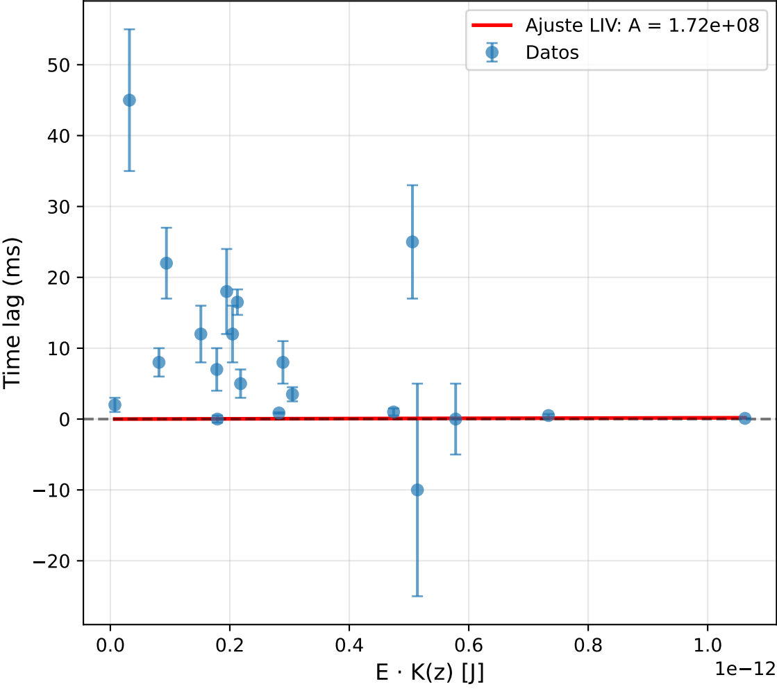
Ajuste modelo LIV \chi^2/\text{dof} = 15.05 , E_{\text{QG}}/E_{\text{Pl}} = 6.8e-01
