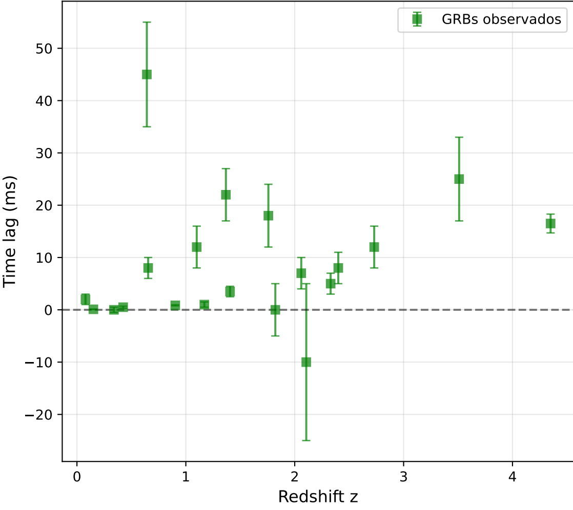
Lag vs Redshift Spearman \rho = 0.467 , p = 0.038
