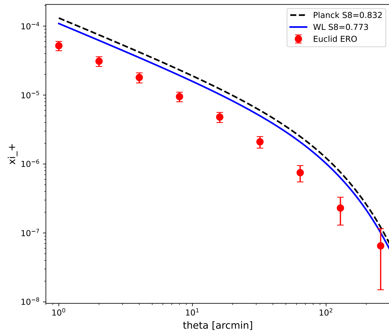
Cosmic Shear Correlation Function
