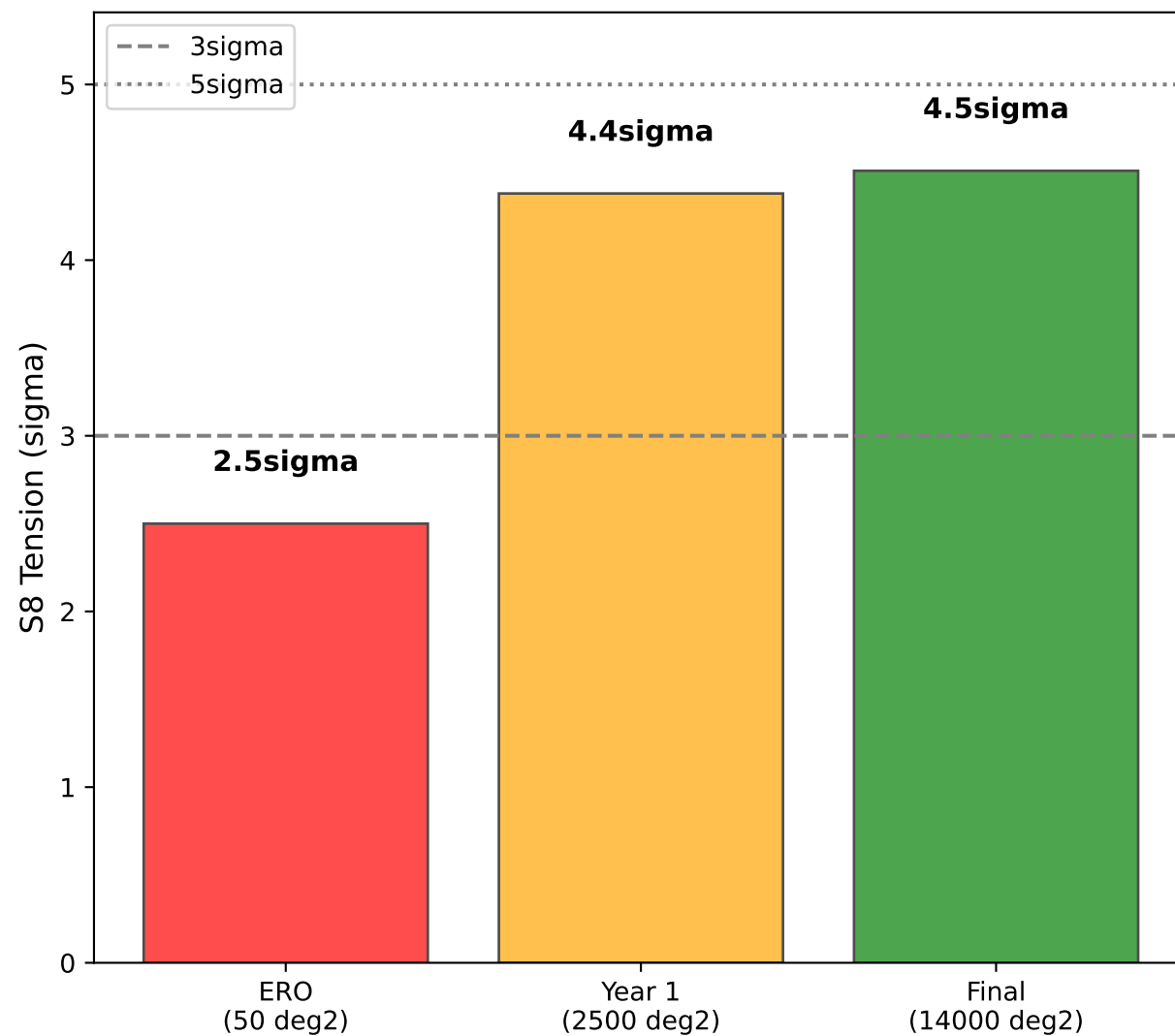
Euclid OCTH Detection Forecast
