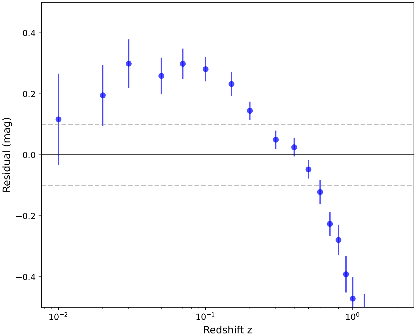
Hubble Diagram Residuals from LCDM
