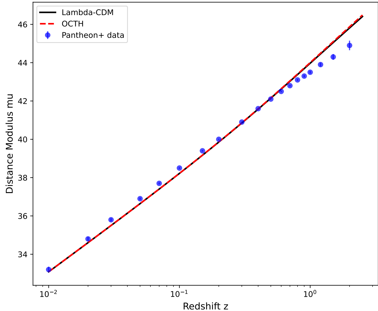
Pantheon+ Hubble Diagram
