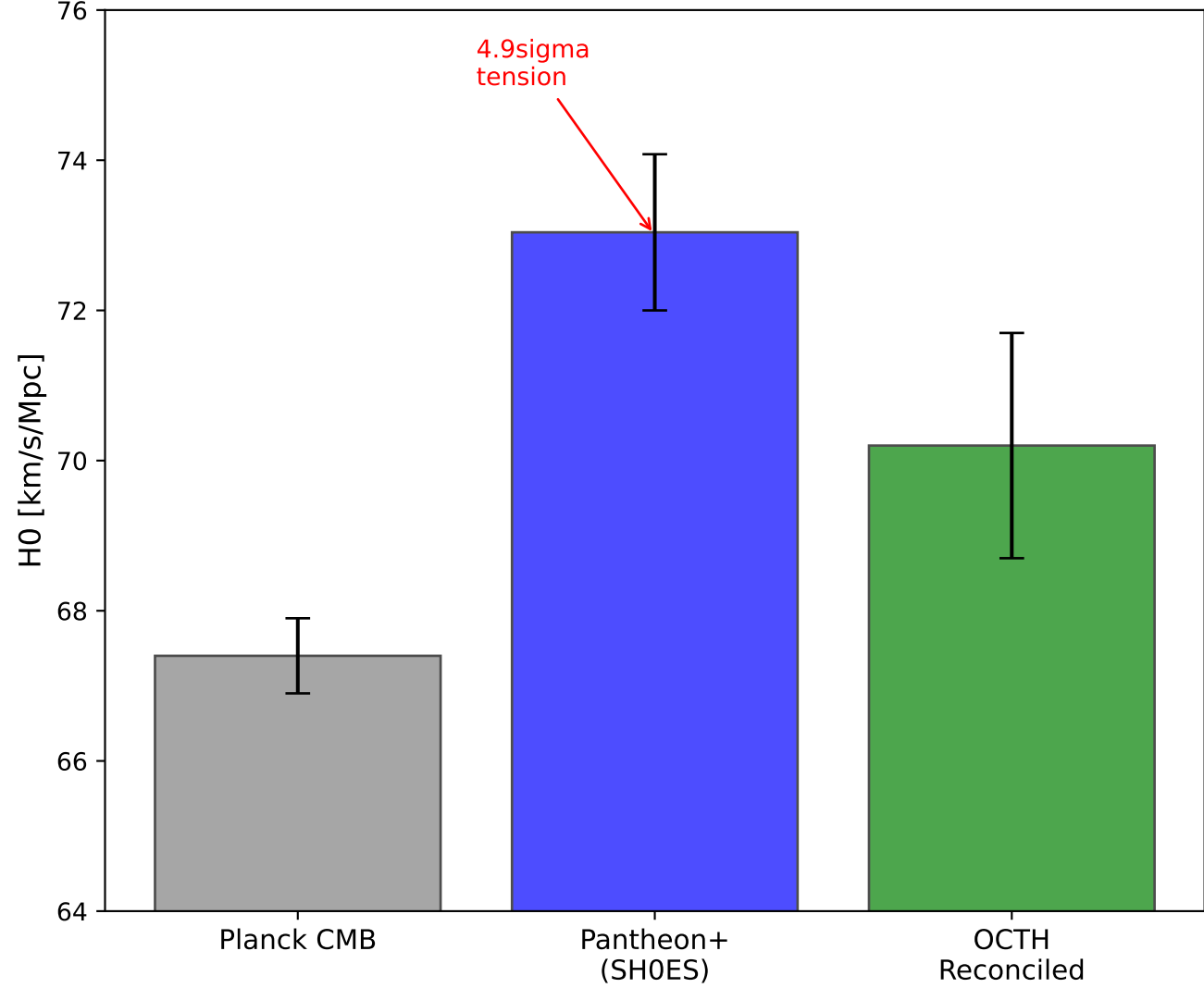
H0 Tension and OCTH Resolution
