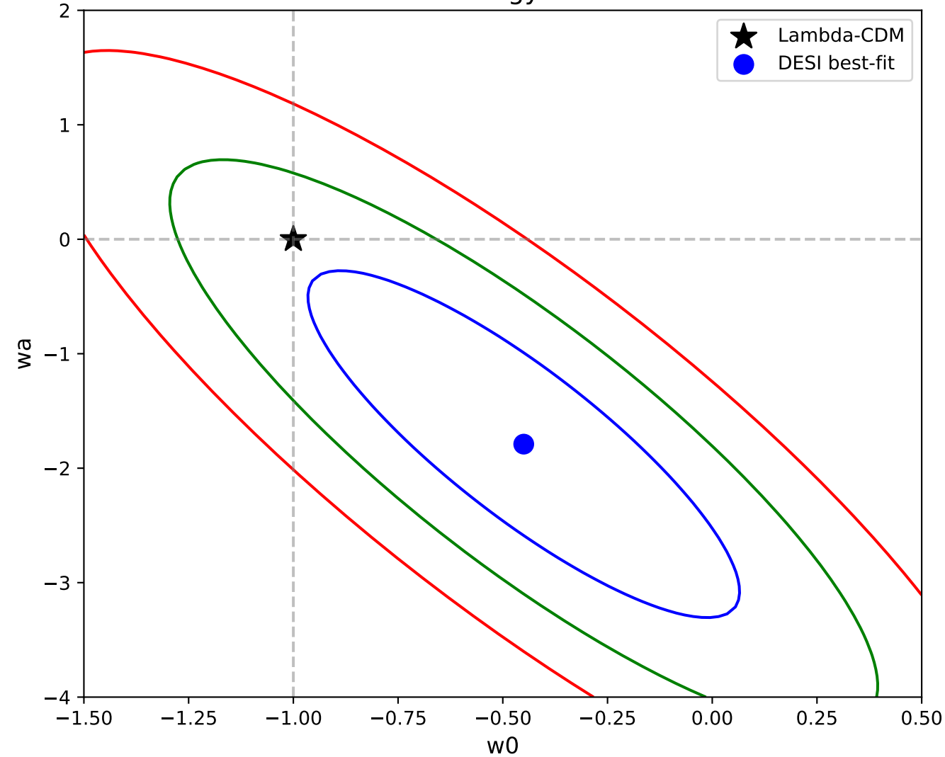
DESI Dark Energy Constraints
