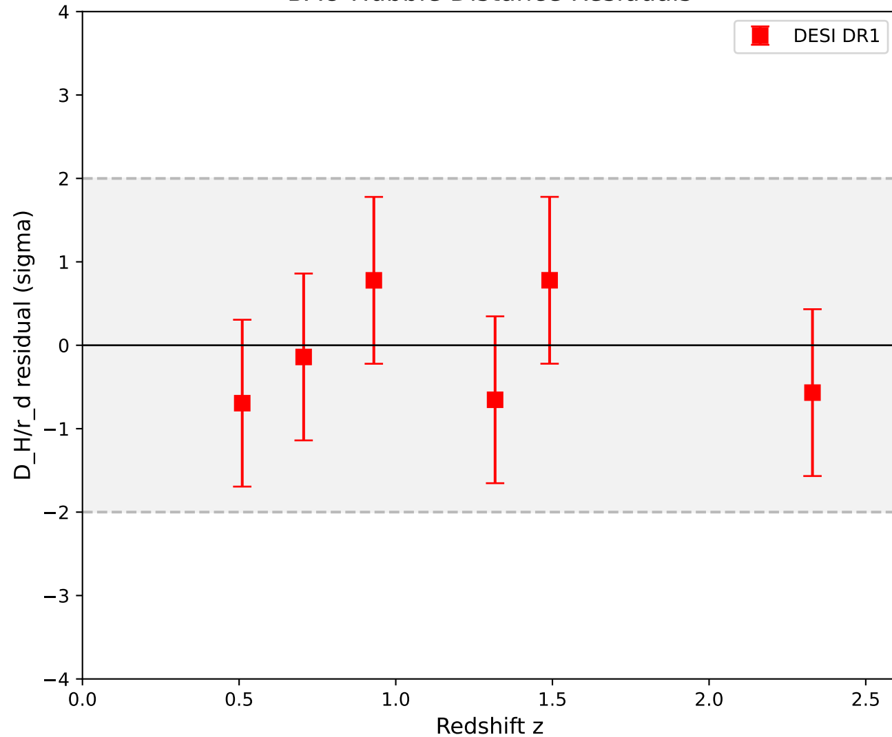
BAO Hubble Distance Residuals
