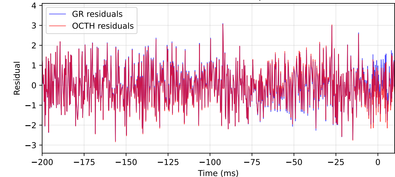
Residuals: Data - Template
