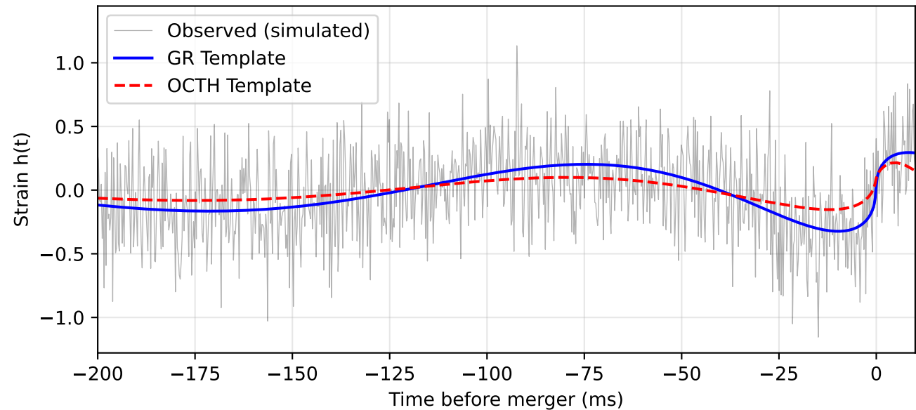
GW150914: Waveform Comparison
