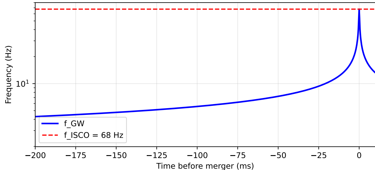
Gravitational Wave Frequency (Chirp)
