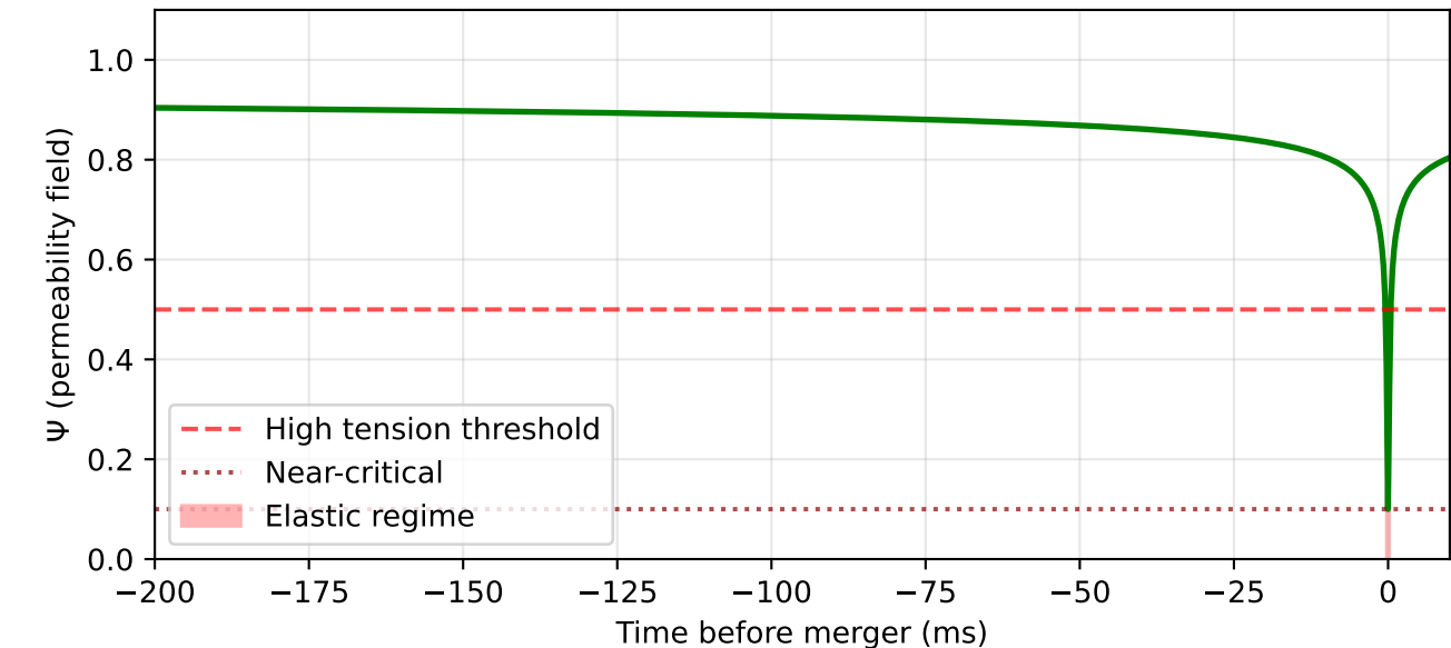
Temporal Permeability During Inspiral
