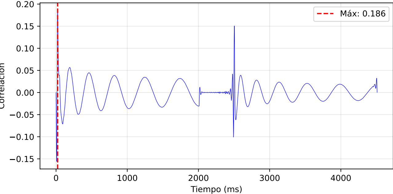
Matched Filter (SNR \approx 16.9)
