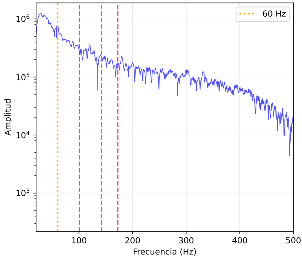
GW151226 f_ISCO = 203 Hz
