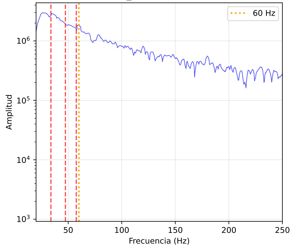
GW150914 f_ISCO = 68 Hz
