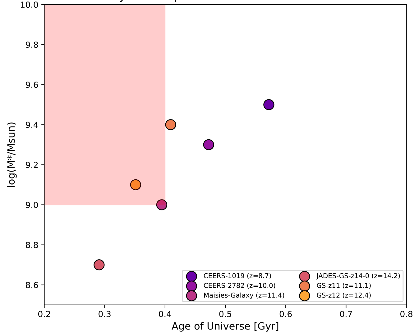
JWST "Impossible" Massive Galaxies
