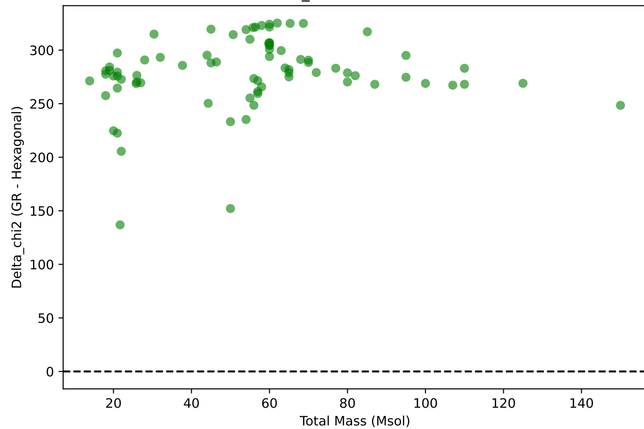
Cumulative Statistical Significance
