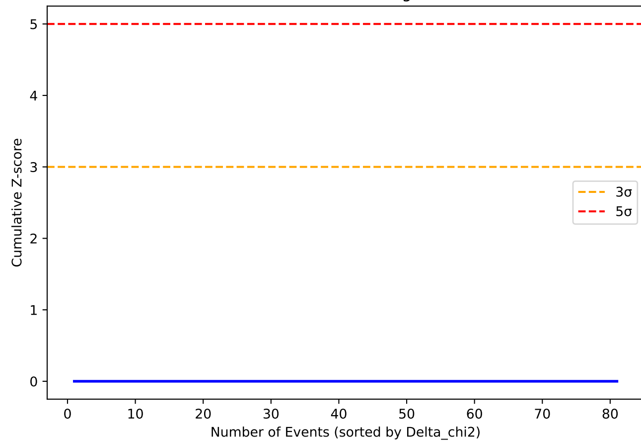
Cumulative Statistical Significance
