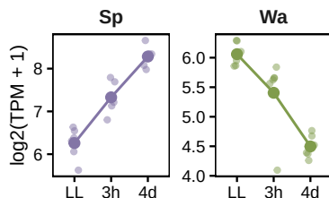
I RPS15A ( p = 2.7e-02 )
