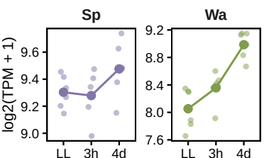
H CYTC-1 ( p = 4.9e-03 )
