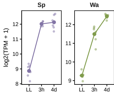
D ORLIKE ( p = 8.2\text{e-}01 )
