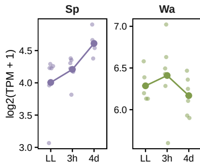
E LCYB ( p = 3.7\text{e-}02 )
