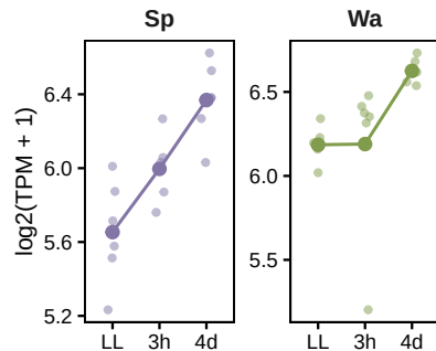
F BCH1 ( p = 8.0\text{e-}01 )
