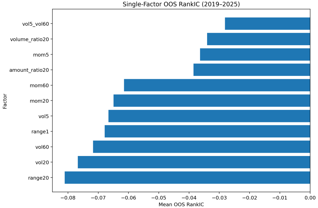
Figure 1: OOS mean RankIC for the eleven frozen single-factor signals. Negative values mean that higher raw signal values predict lower subsequent returns.
