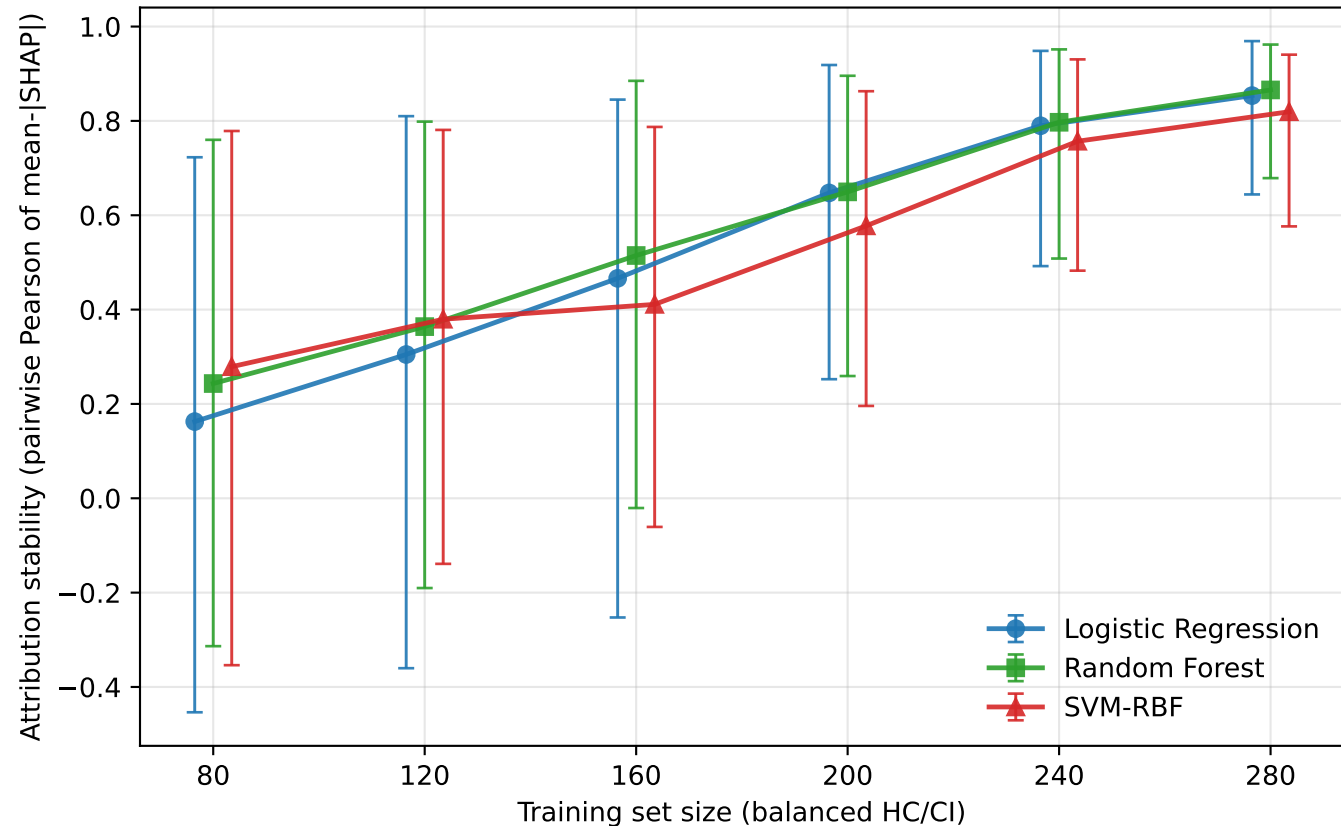
SHAP attribution stability vs. training size
