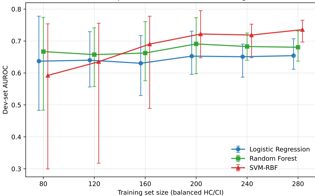
Predictive performance (AUROC) vs. training size
