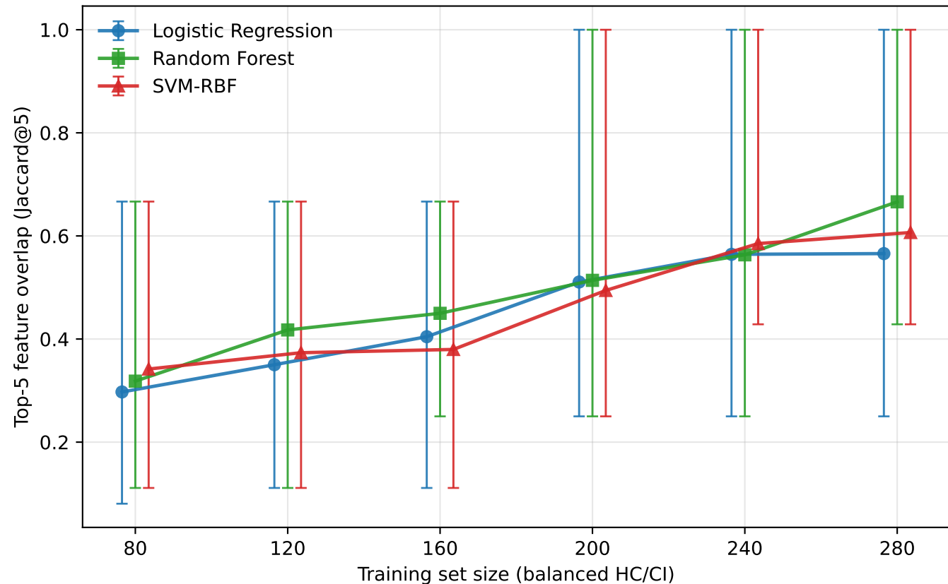
Top-5 SHAP feature-set stability vs. training size
