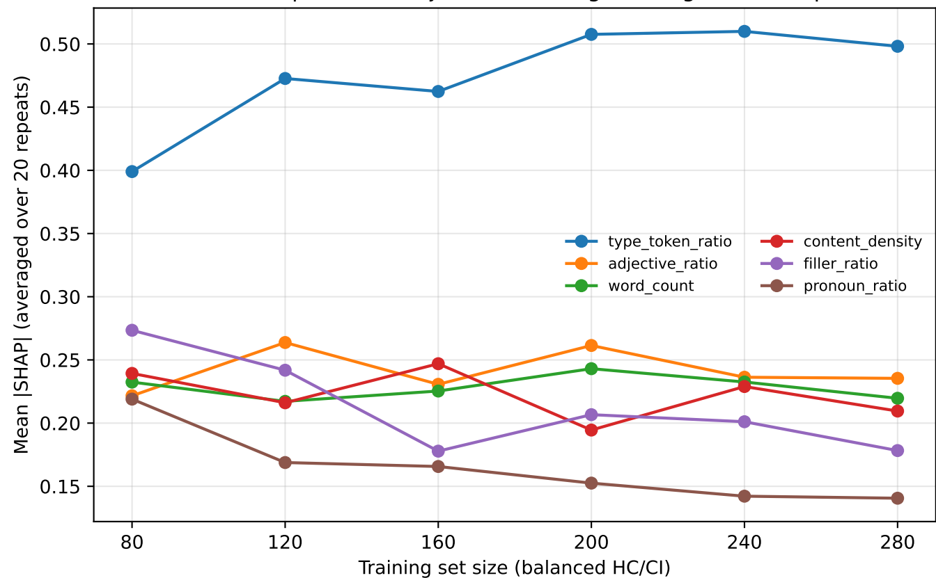
Feature-importance trajectories — Logistic Regression (top 6)
