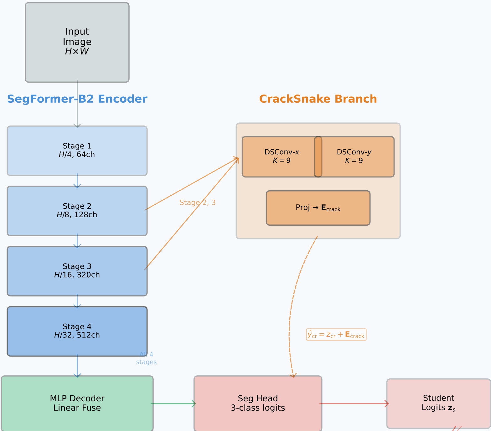
(a) SegFormer-DSConv Architecture
