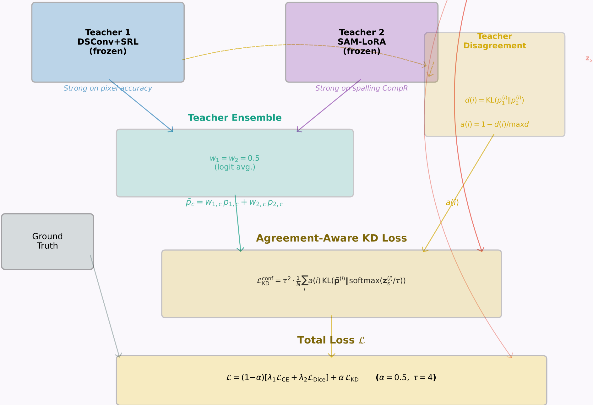
(b) Dual-Teacher KD (DTKD)
