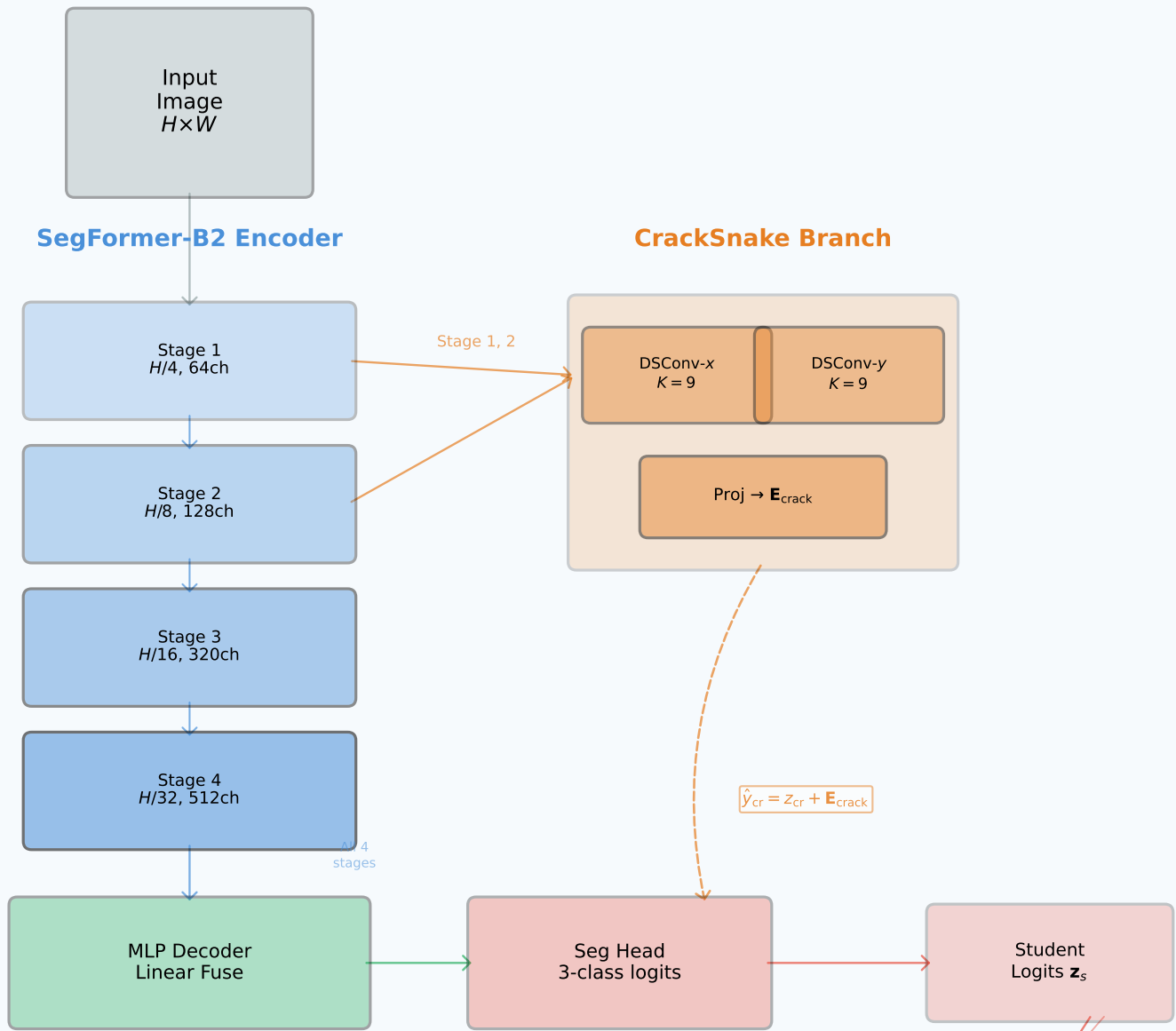
(a) DSCFormer Architecture
