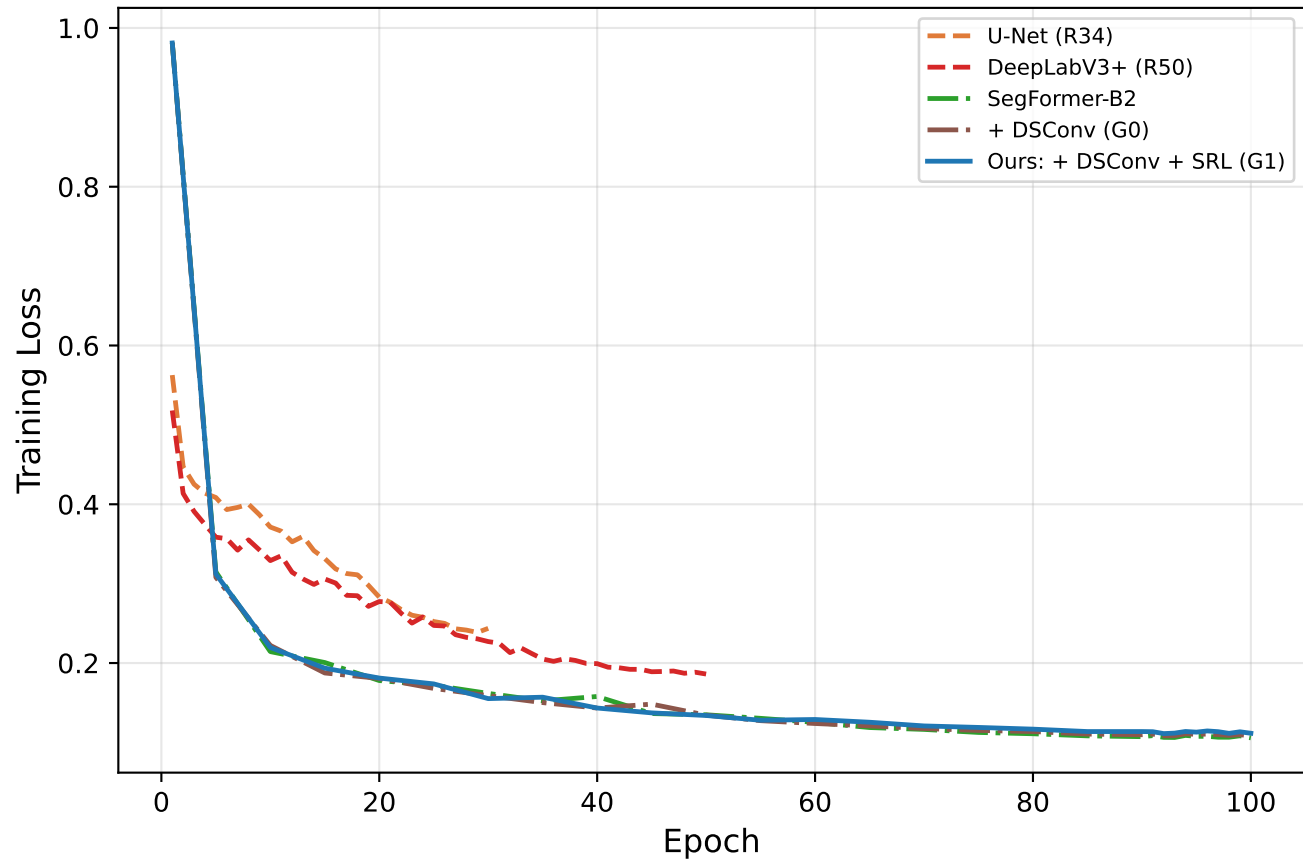
(b) Training Loss
