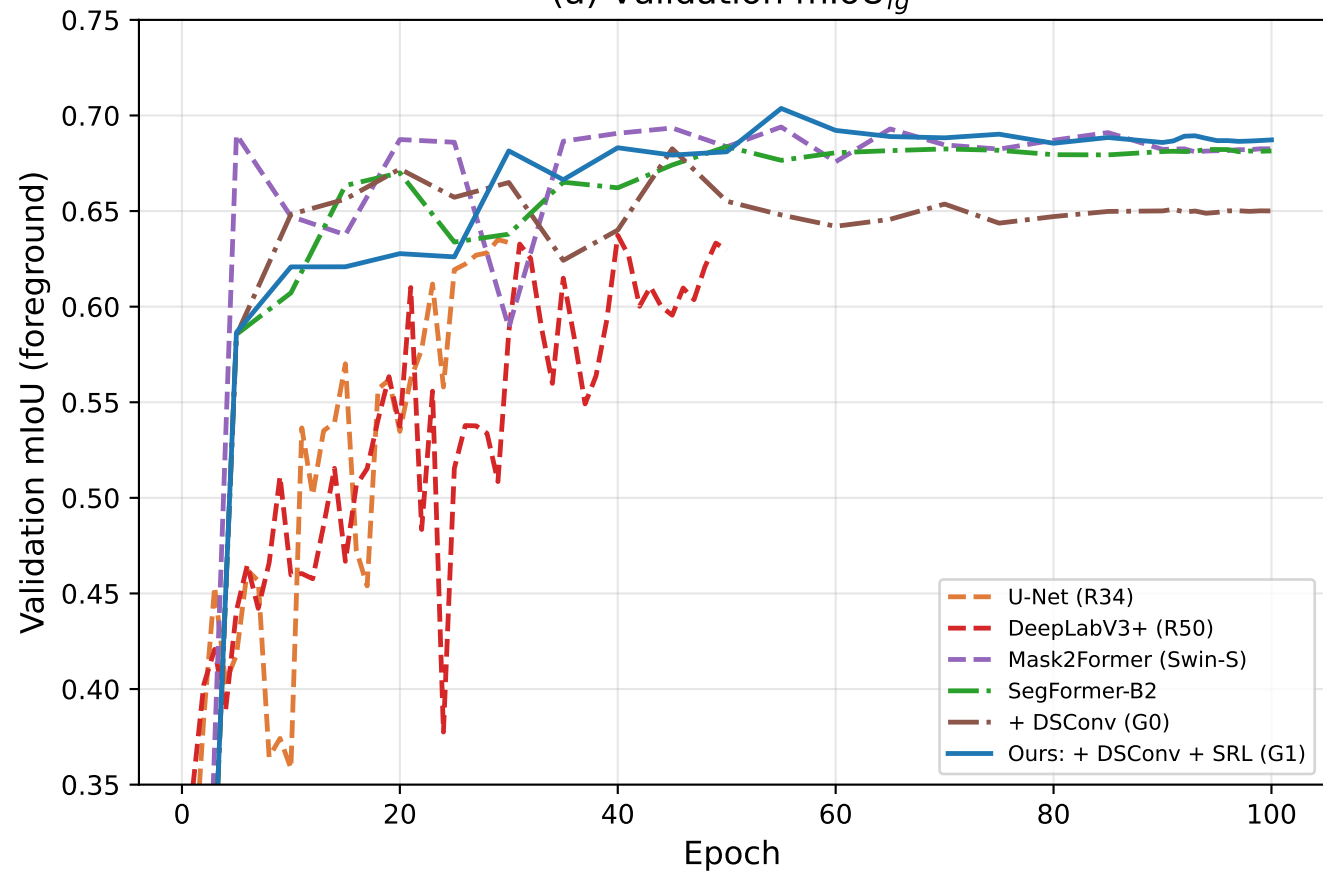
(a) Validation mIoU fg
