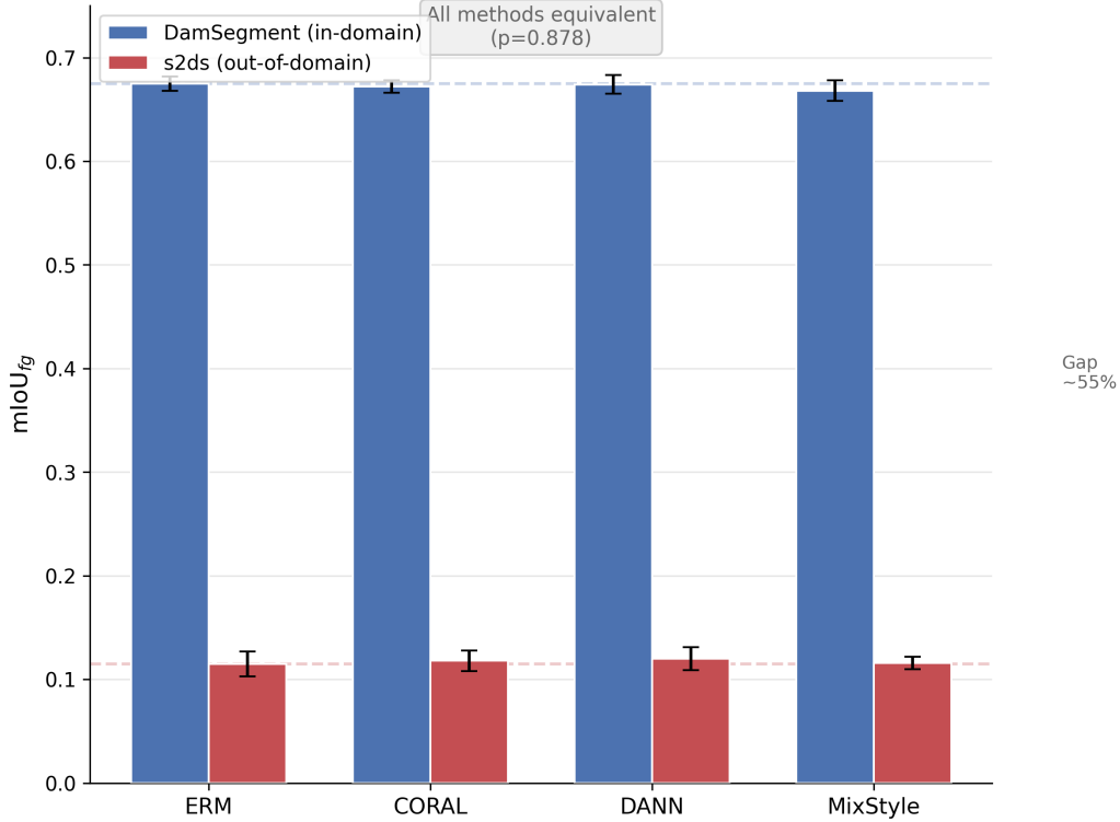
Figure 5: Domain generalisation results across 3 seeds on in-domain (DamSegment) and out-of-domain (s2ds) evaluation. All methods achieve similar in-domain ( \sim 0.67 mIoU fg ) and OOD ( \sim 0.12 mIoU fg ) performance, with a stable domain gap of \sim 55\% . Dashed lines indicate ERM baseline means.
