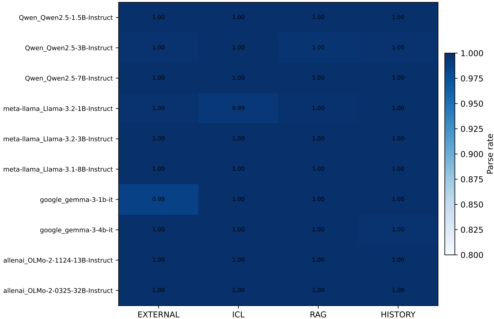
Ablation Parse Rate by Model × Suite
