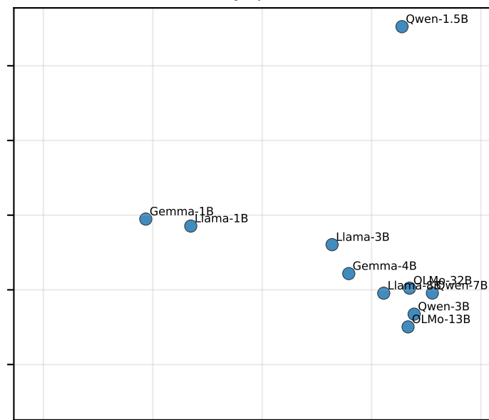
History \rho=-0.64
