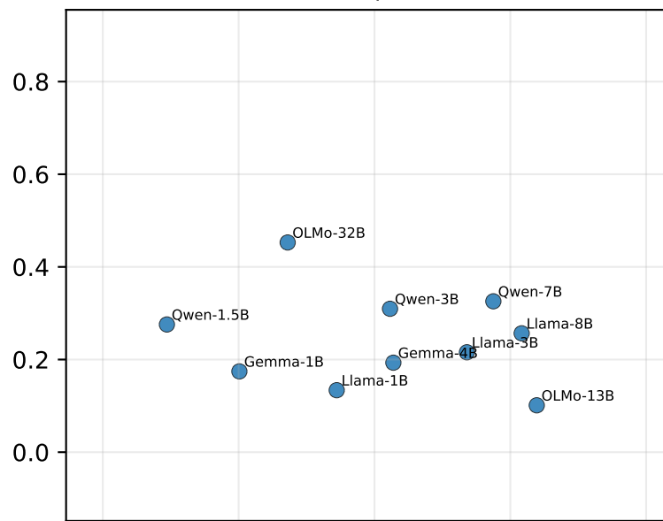
External \rho=-0.20
