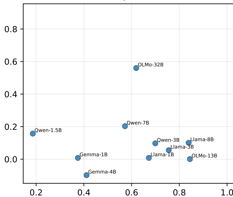
RAG \rho=-0.13
