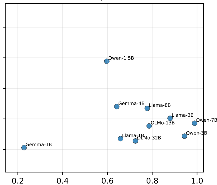
Tool \rho=0.03
