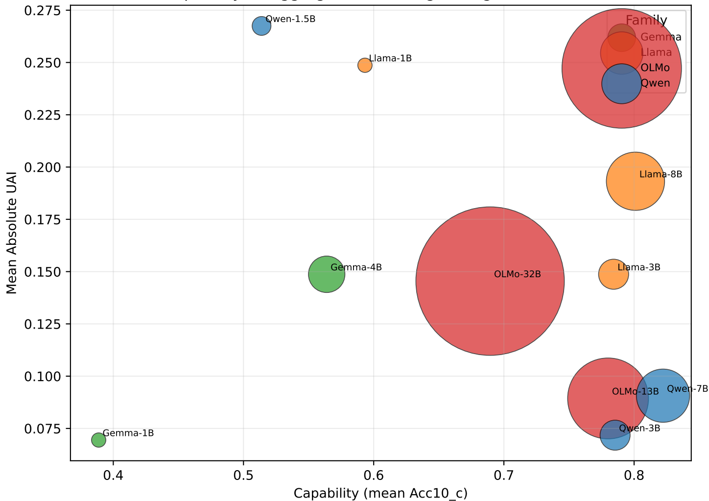
Capability vs Aggregate Anchoring Strength (All Suites)
