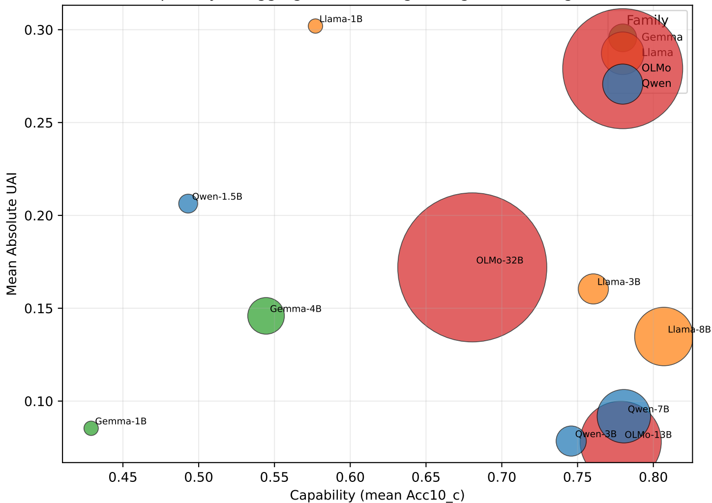
Capability vs Aggregate Anchoring Strength (Excluding Tool)
