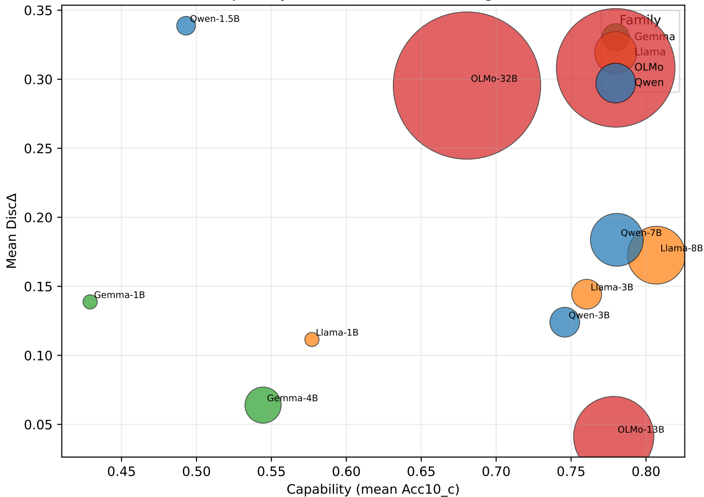
Capability vs Mean Disc \Delta (Excluding Tool)
