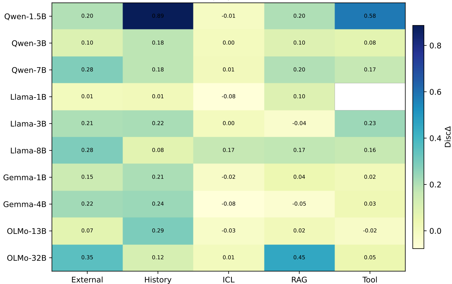
DiscΔ Heatmap by Model and Suite
