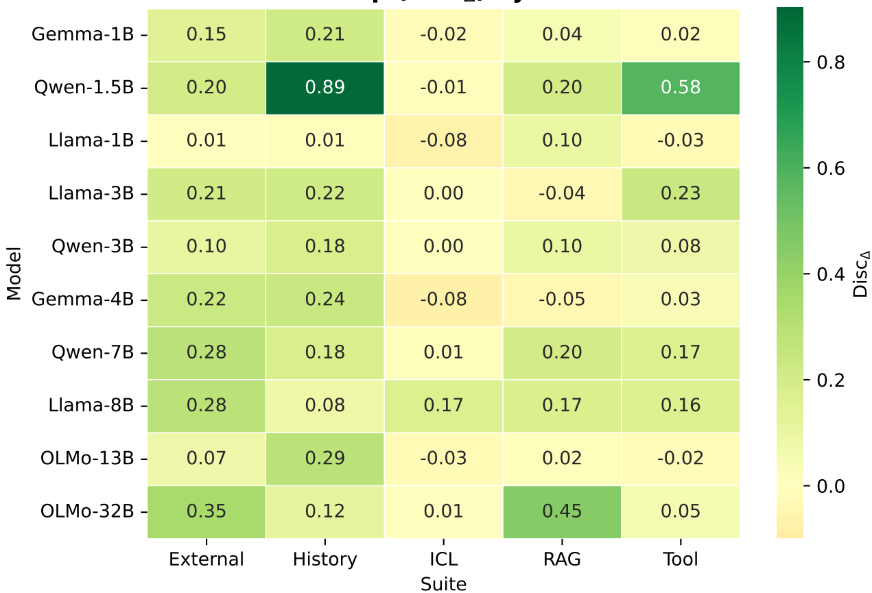
Discrimination Gap (Disc Δ ) by Model and Suite
