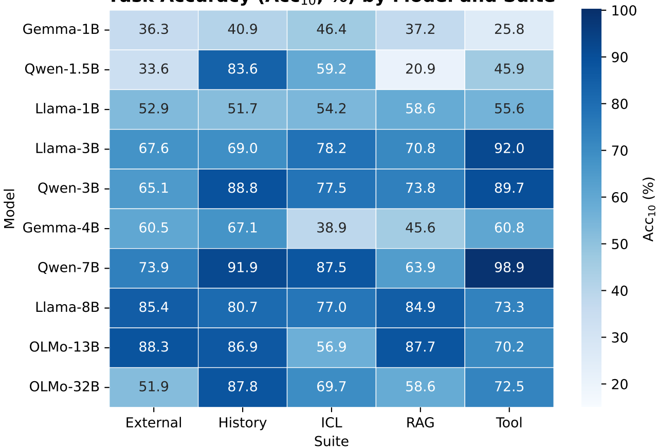
Task Accuracy (Acc 10 , %) by Model and Suite
