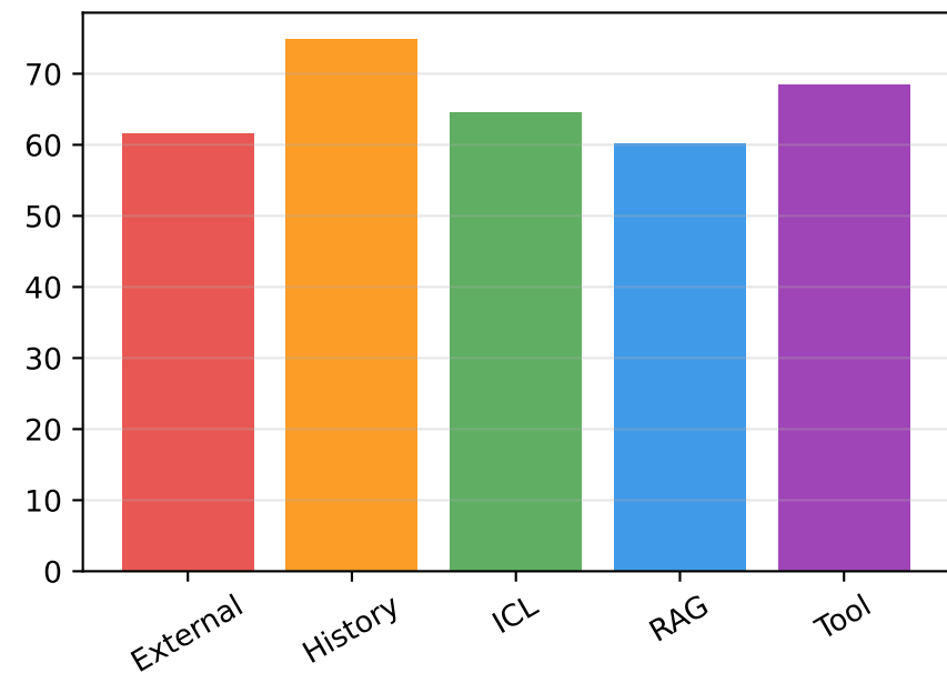
Mean Acc_{10} (%)
