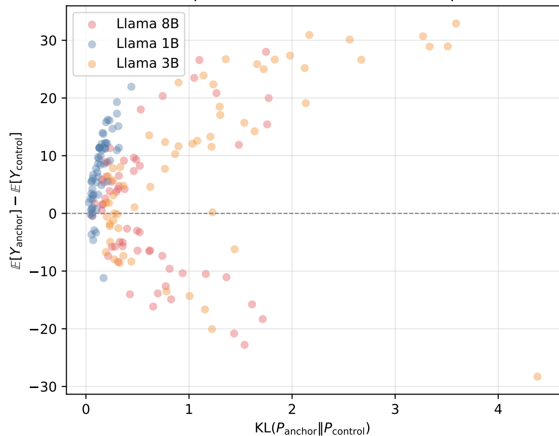
Anchor Imprint: Distributional Shift vs Output Bias
