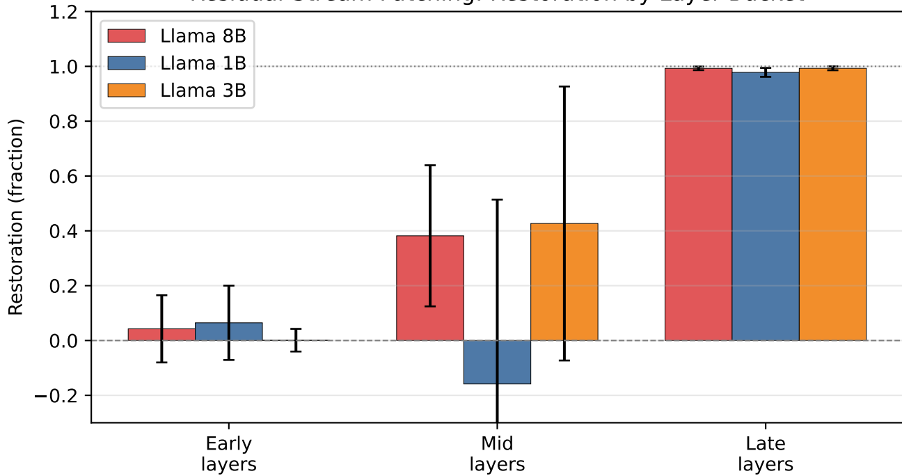
Residual-Stream Patching: Restoration by Layer Bucket
