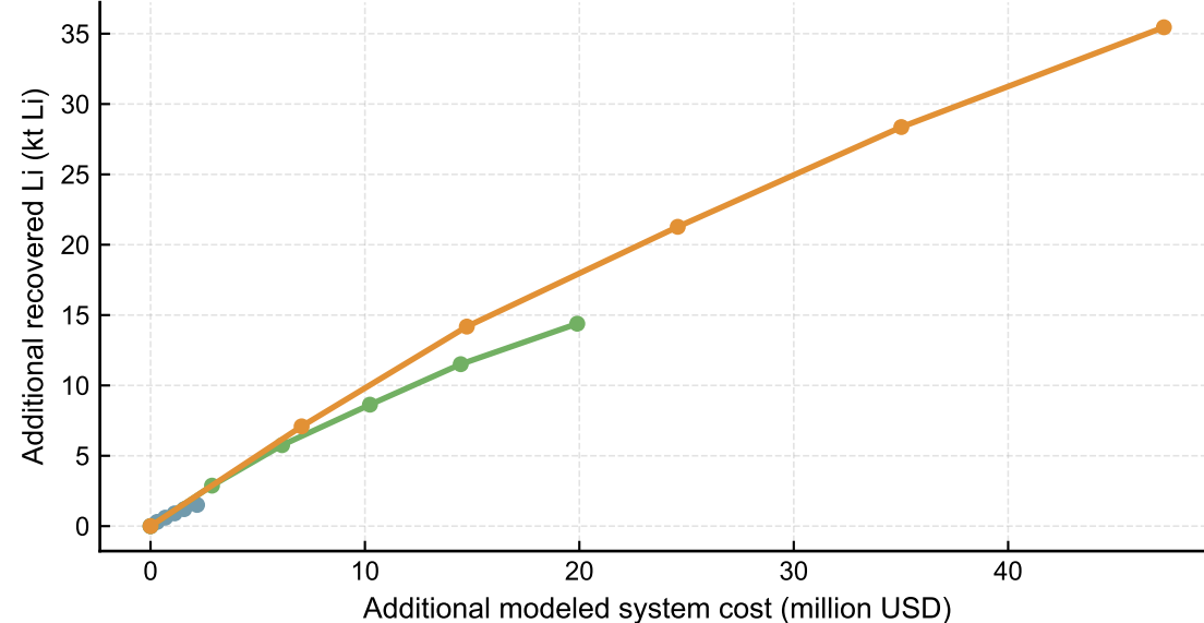
C. Pareto frontier: extra Li requires additional cost
