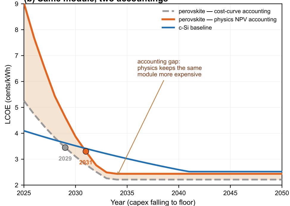
(b) Same module, two accountings
