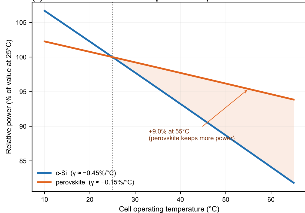
(a) Device cause: the two temperature slopes
