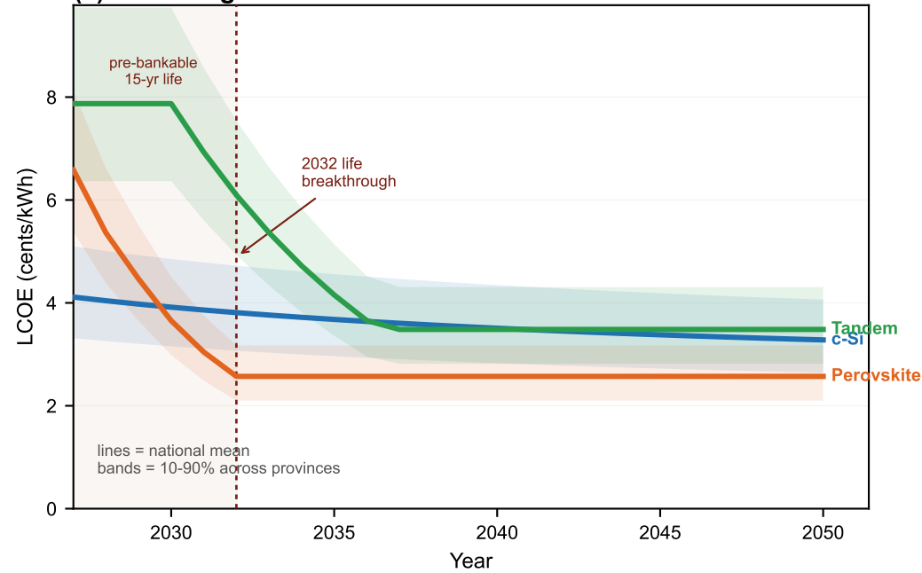
(a) Lifetime gate in LCOE
