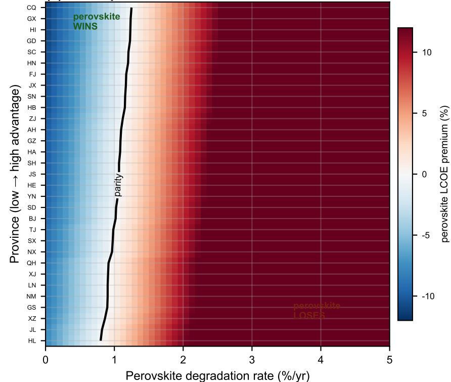
(a) LCOE premium surface vs c-Si
