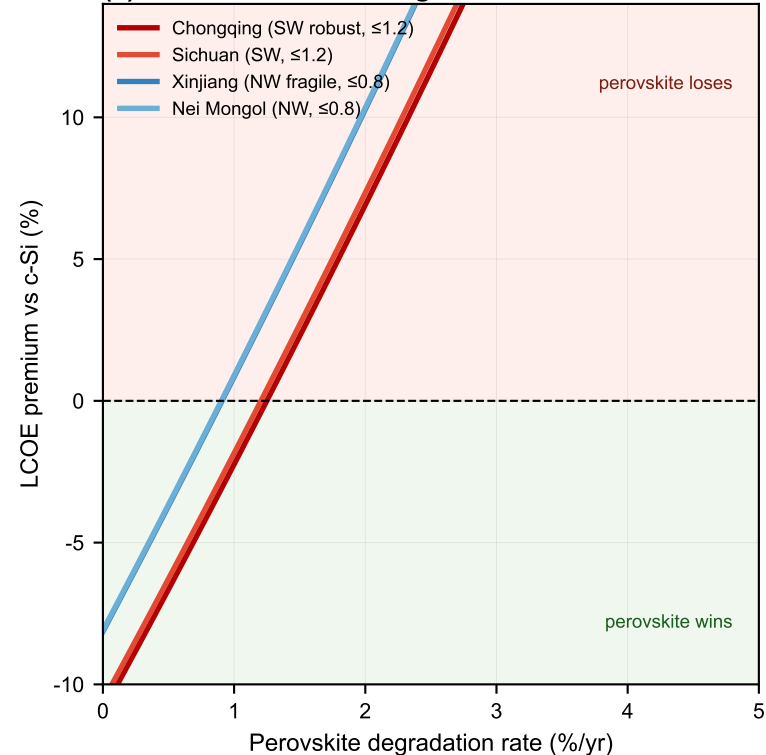
(c) SW absorbs more degradation than NW
